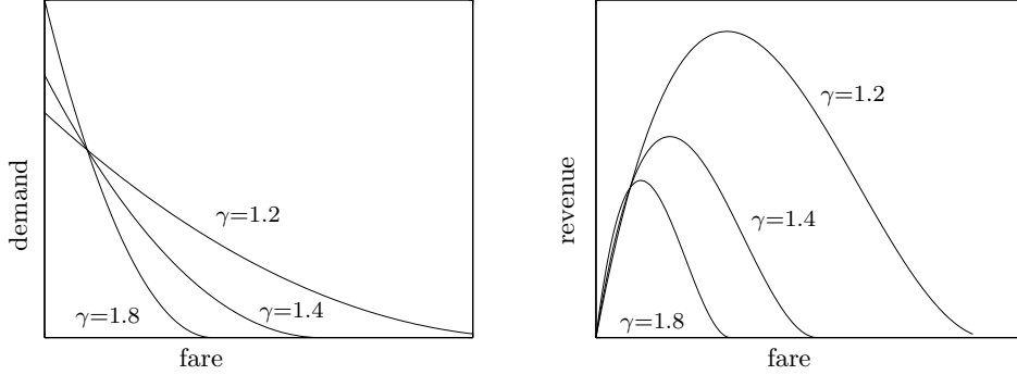
Figure 1: Left: Sketch of quadratic demand function (2) for different values of \gamma . Right: Resulting revenue functions.
