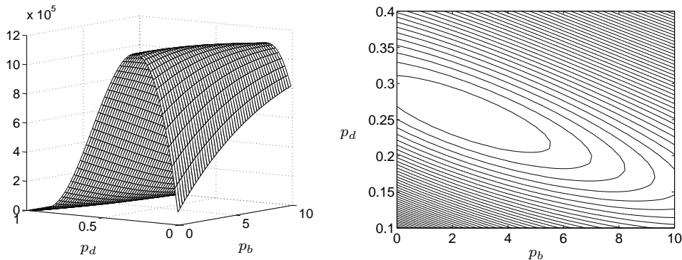
Figure 2: Textbook example. Left: Total revenue. Right: A contour plot of the total revenue. The optimum is at p_b \approx 2.29 and p_d \approx 0.26 .
