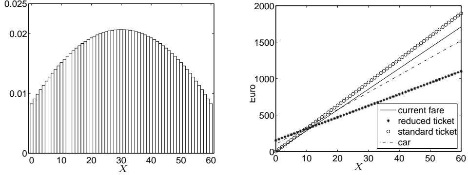
Figure 3: Left: The discrete random variable X for the number of trips. Right: Example of fares in dependence on the number of trips for a selected OD-pair (s, t) of high distance.
