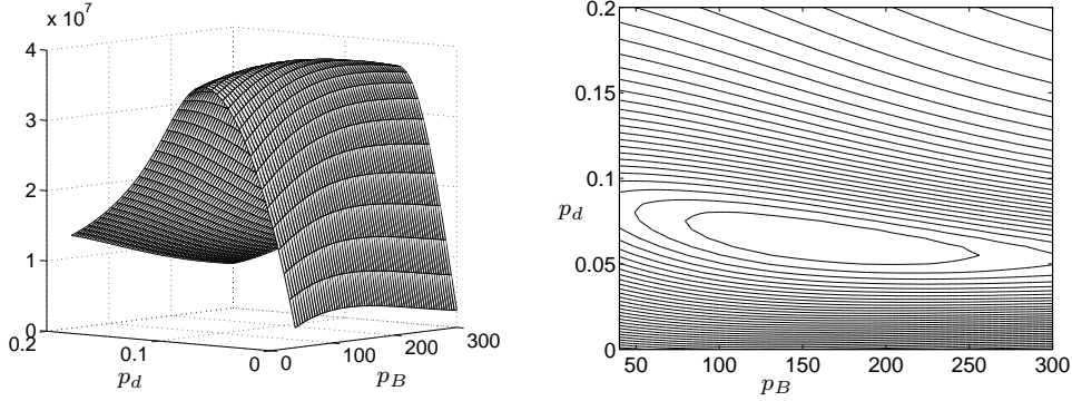
Figure 4: Discrete choice model. Left: Total revenue. The optimum is at p_B \approx 153.30 and p_d \approx 0.06 . Right: A contour plot of the total revenue.
