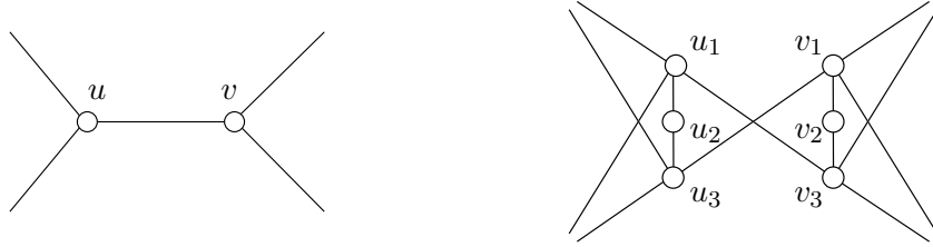
Figure 1: Example for the node splitting in the proof of Proposition 4.1
