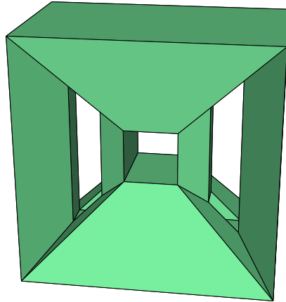
FIGURE 10. The surface Q_5 of genus 5, realized in \mathbb{R}^3 ( polymake/javaview graphics by Thilo Schröder); compare the figure in McMullen, Schulte & Wills [18, p. 300]!
