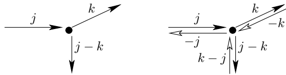
FIGURE 4. The flow condition, “Kirchhoff’s law.” The left figure shows how a flow of size j is split into two parts. In the right figure the reversed arcs have been added: This contains the same amount of information, but the data can be read off more directly.
