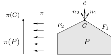
FIGURE 11. The normal vector c for the face G can be written as a positive combination of the normal vectors of the faces F_1, F_2 that contain G . The face G \subset P is strictly preserved by the projection of P to the second coordinate.
