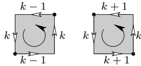
FIGURE 9. The orientation of Q_m described in the text; here the black vertices are the ones with an even sum of coordinates.
