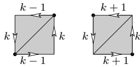
FIGURE 12. The triangulation of Q_m described above. Here we assume that k is even. The black vertices are the ones with an even sum of coordinates.
