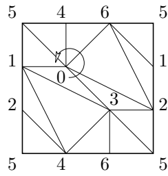
FIGURE 3. The Möbius torus. Read off the rotation scheme from this sketch!
