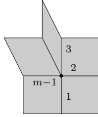
FIGURE 8. The star of a vertex in Q_m
