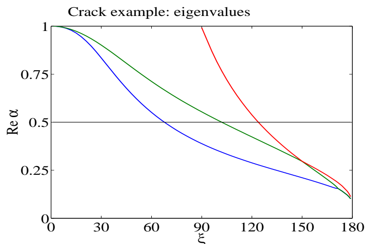
Fig. 4 Real part of the interesting eigenvalues against the angle \xi .
