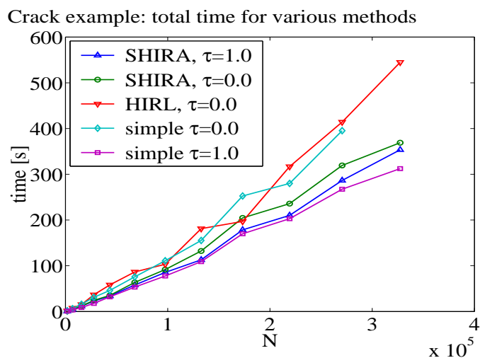
Fig. 5 CPU times for crack with \xi = 120^\circ and various N .
