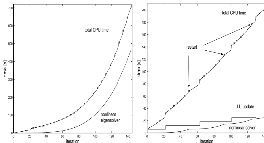
Fig. 2 Arnoldi method without and with restarts
