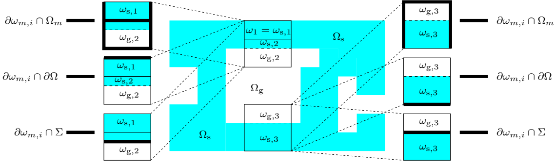
Figure 4: Illustration of the decomposition of the boundary of control volumes \omega_{m,i} according to (3.5a). The lower control volume \omega_3 is not admissible, as it has 2-dimensional intersections with both \Sigma and \partial\Omega (see Rem. 3.1).
