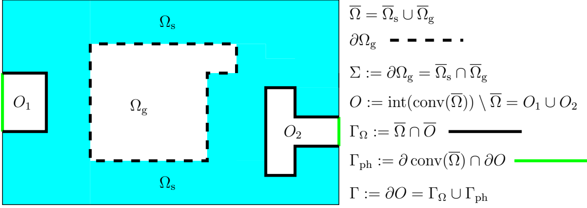
Figure 2: For the domain of Fig. 1, the surfaces of radiation regions are shown. The open radiation regions O_1 and O_2 are artificially closed by the phantom closure \Gamma_{\text{ph}} . As in Fig. 1, Fig. 2 depicts a 2-dimensional section through the 3-dimensional domain.
