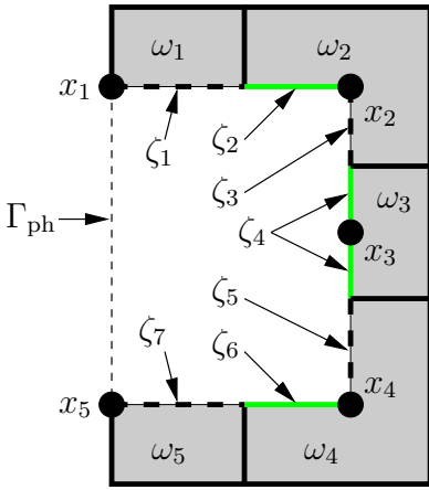
Figure 6: Magnification of the open radiation region O_1 and of the adjacent part of \Omega_s (cf. Figures 1, 2). It illustrates the partitioning of \Gamma_\Omega into the \zeta_\alpha . In particular, it illustrates the compatibility condition (DA-7) as well as Def. and Rem. 3.2.
