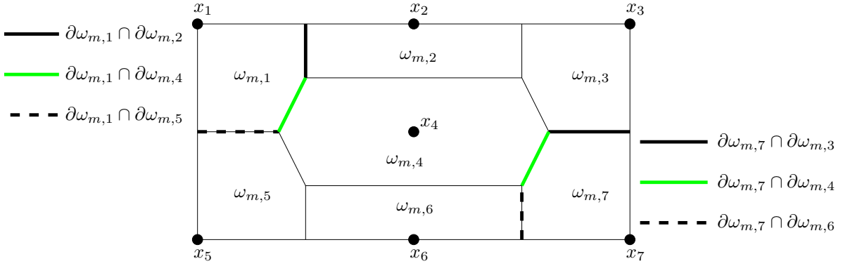
Figure 5: Illustration of conditions (DA-4) (with \Gamma_\Omega = \emptyset ) and (DA-5) as well as of the partition of \partial\omega_{m,i} \cap \Omega_m according to (3.8). One has \text{nb}_m(1) = \{2, 4, 5\} and \text{nb}_m(7) = \{3, 4, 6\} .
