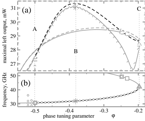
Figure 5: Path following of the periodic orbit. a: maximal output at the left facet. b: frequency of pulsations. Solid, dashed lines and empty bullets are due to 4MA, 3MA and full TW model, respectively. Black and grey lines show stable and unstable orbits in MA systems. Squares and triangles represent torus and fold bifurcations, respectively. The stars at the \phi = B indicate the orbits considered in Fig. 4.
