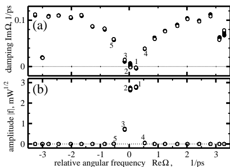
Figure 3: Mode analysis of the pulsating regime of the TW model. Empty and full bullets show the main eigenvalues \Omega (panel a) or the modulus of the mode amplitude |f| versus their frequency (panel b) at fixed t or all time moments, respectively.
