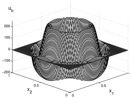
FIG. 5.2. Control u_h in the first example.
