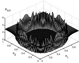
FIG. 5.5. Lagrange multiplier \mu_{a,h} .
