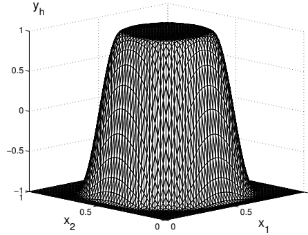
FIG. 5.3. State y_h in the first example.
