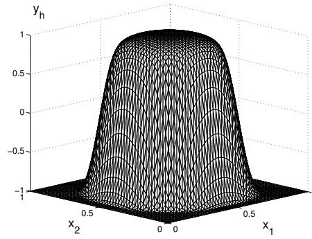
FIG. 5.8. State y_h in the second example.
