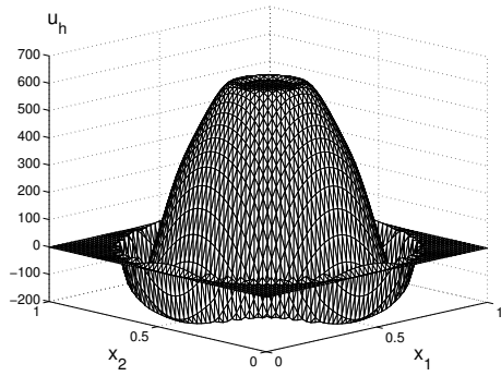
FIG. 5.7. Control u_h in the second example.
