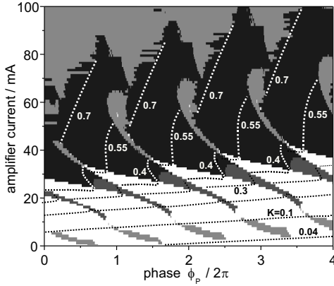
Figure 3: Calculated areas of self-pulsations in the plane spanned by the two parameters \phi_P and I_A . The DFB injection level was fixed to I_{\text{DFB}} = 70 mA, the damping in the phase section is increased by 5/cm per 2\pi . White areas correspond to cw output. Different levels of grey indicate non-stationary output with frequencies f (main peak of power spectrum) in the following ranges: f < 15 GHz (light), 15 GHz < f < 30 GHz (dark), and f > 30 GHz (black). Dotted lines represent curves of constant K (averaged over one pulsation period in the self-pulsation areas).
