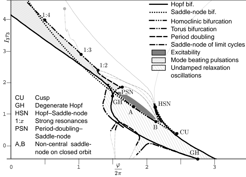
Figure 2: Bifurcation diagram for the two-mode approximation (truncated (15) with q = 2 ) in the parameter plane (\varphi, I_3) (see [26] for the particular parameter values).
