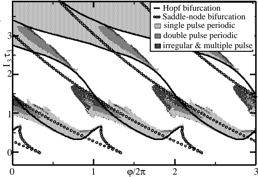
Figure 3: Parameter study of a three section laser by direct simulation of PDE model with LDSL-tool. Full model and used parameter values (except of l_1 = 250 \mu\text{m} , l_2 = 400 \mu\text{m} and \alpha = 15 \text{ cm}^{-1} ) can be found in [26].
