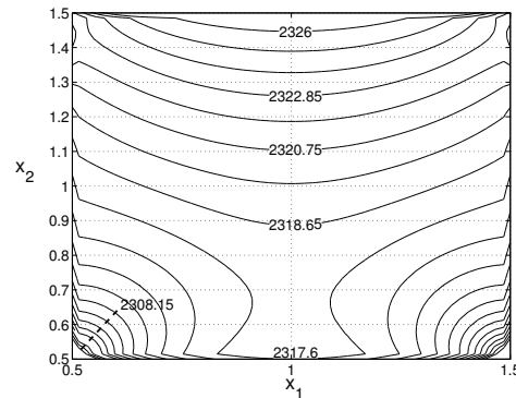
FIG. 8.9. Isotherms in the gas phase \Omega_g .
