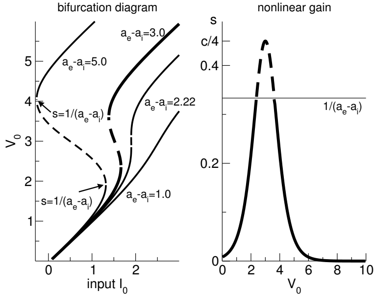
Fig. 2. Bifurcation diagram and nonlinear gain for constant bifurcations for a_e > a_i . Left panel: Stability of the stationary state V_0 with respect to external input I_0 . For a_e - a_i > 4/c = 2.22 , both stable (solid line) and unstable branches (dashed line) exist, while for a_e - a_i \leq 2.22 there is only a single stable solution. Right panel: The nonlinear gain s with respect to the constant state V_0 . The horizontal line s = 1/(a_e - a_i) separates stable from unstable states and determines the critical values of V_0 . In both panels, we applied the sigmoid function introduced in Fig. 1.
