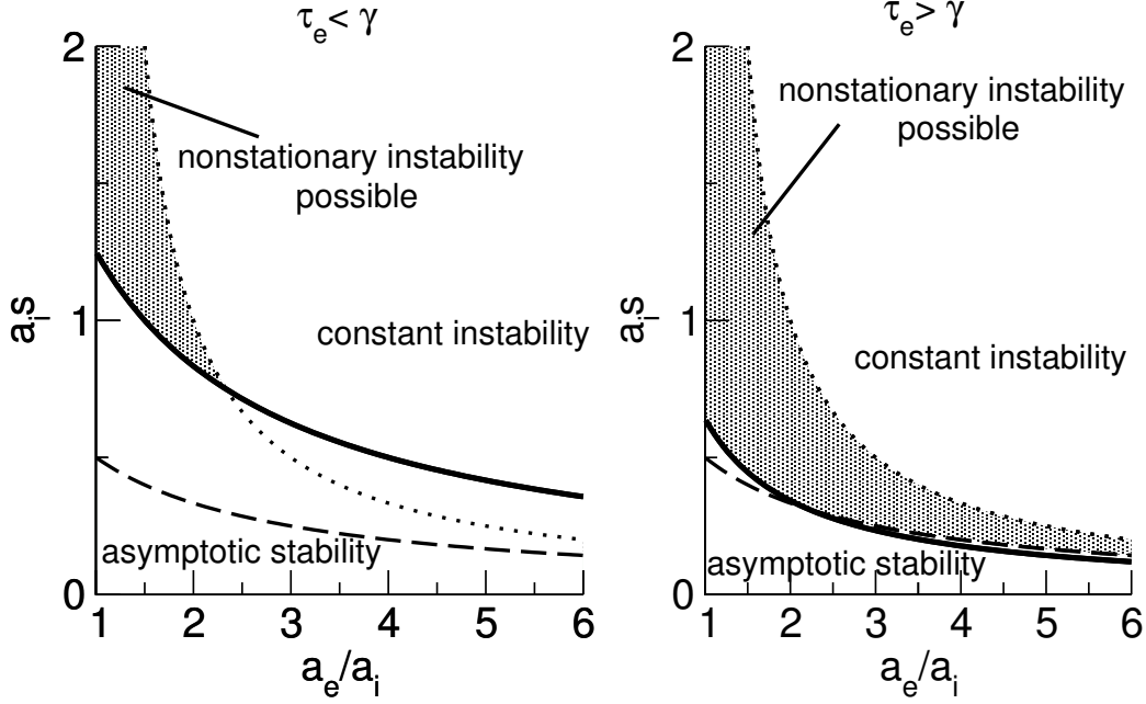
Fig. 3. Necessary parameter regime for nonstationary instabilities for diverse mean excitatory interaction time \tau_e and synaptic delay constant \gamma . Valid parameters (hatched area) are constrained by the threshold of Eq. (18) plotted as solid line, the threshold of constant bifurcation (dotted line) and the threshold of asymptotic stability (dashed line).
