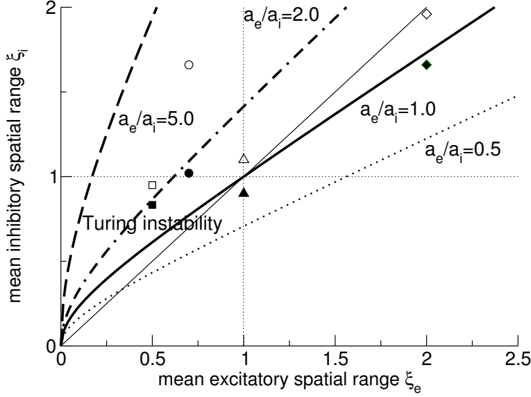
Fig. 8. Sufficient parameter regimes of Turing patterns with respect to spatial interaction ranges \xi_i , \xi_e and various values of a_e/a_i . The thin solid line denotes \xi_i = \xi_e , while filled and empty squares, triangles and diamonds mark different cases discussed in Figs. 9 and 10.
