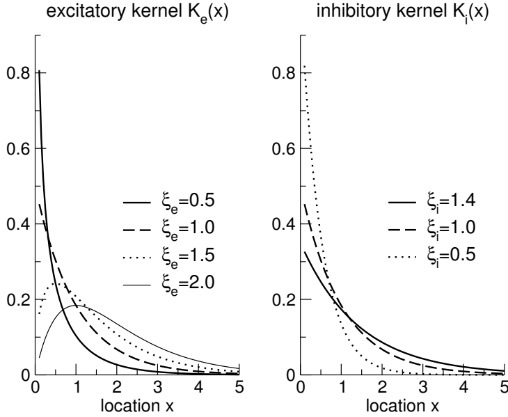
Fig. 7. Excitatory and inhibitory kernels for various parameters. All kernels are finite except for K_e(x) for p = 0.5 . In case of \xi_e > 1 , the excitatory kernel K_e(x) exhibits a maximum at x = \xi_e - 1 . We point out that \xi_e < 1 yields divergent excitatory self-connectivity, while the excitatory self-connectivity vanishes for \xi_i > 1 .
