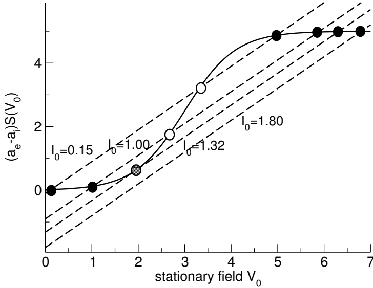
Fig. 1. Illustration for the detection of constant stationary solutions of Eq. (8). For I_0 < 1.32 , there are three solutions, while for I_0 > 1.32 there is only a single one at large values of V_0 . Simple iteration studies near the solutions reveal their stability: Filled circles represent stable fixed points, while empty circles illustrate unstable fixed points. At the critical value I = 1.32 , there is a saddle node solution (hatched circle) synchronous to a stable fixed point at large values of V_0 , cf. Fig. 2. Here, we applied the sigmoid function S = 1/(1 + \exp(-c(V - V_r))) [35,43], a_e = 10 , a_i = 5 and c = 1.8 , V_r = 3.0 [44].
