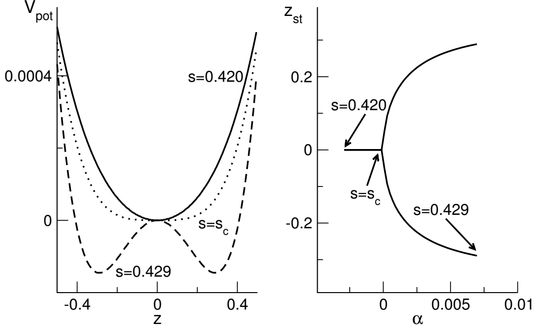
Fig. 6. Potential V_{pot} and bifurcation diagram of the order parameter equation (33). It has been found that k_c = 0.6 , s_c = 0.423 and V_0 = 2.723 at s_c with parameters a_e = 6.0 , a_i = 5.0 , \xi_e = 1.0 , \xi_i = 2.0 , \gamma = 2.1 and the sigmoid function from Fig. 1.
