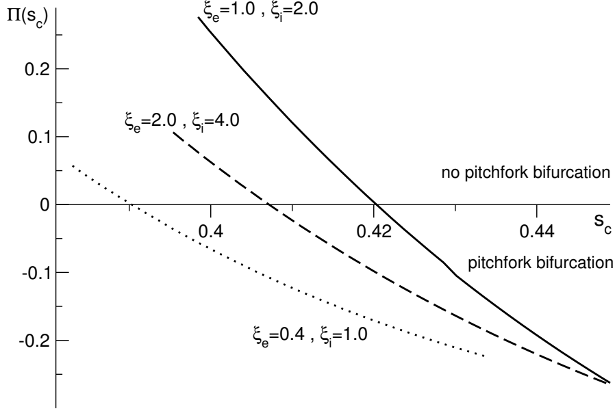
Fig. 5. The factor \Pi of the cubic term in Eq. (33) plotted with respect to the bifurcation threshold s_c from Eq. (15) for various \xi_e, \xi_i . Each suitable parameter set a_e, a_i, \xi_e, \xi_i maps to a maximum of \hat{K}(k) and thus a single value s_c . Thus the plots have been computed by decreasing a_e leading to increasing s_c , while 0 < a_e - a_i < 4/c . The range of a_e depends on \xi_e, \xi_i . The parameters have been chosen as a_i = 5.0 , \gamma = 2.1 and the sigmoid function is as in Fig. 1.
