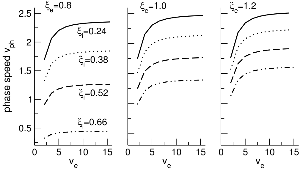
Fig. 11. Plots of the traveling wave speed v_{ph} with respect to the transmission speed v_e for various parameters \xi_e, \xi_i . For \xi_e < 1 , the field reveals traveling waves for local excitation and lateral inhibition, which strongly contrasts to previous findings. The plots show an increase of v_{ph} by decreasing the inhibitory range \xi_i and increasing the excitatory range \xi_e . The applied parameters are a_e = 60 , a_i = 55 , v_i = 100 and \gamma = 2.1 .
