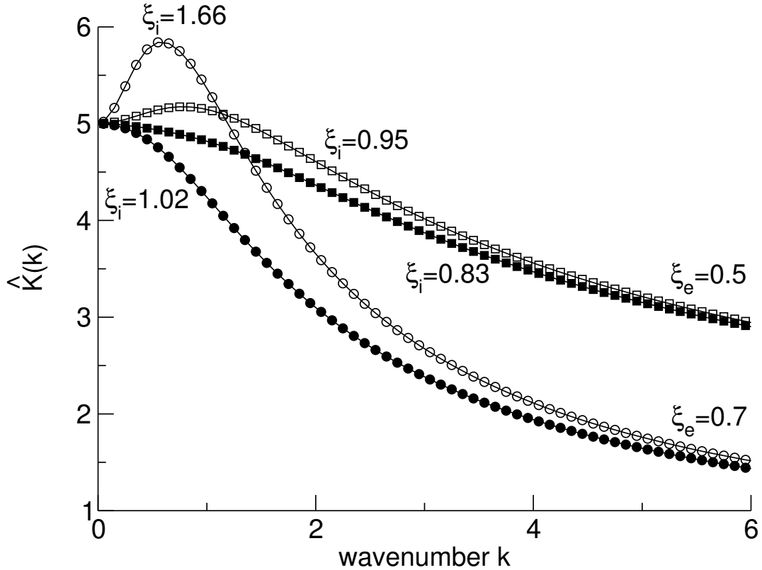
Fig. 9. Function \hat{K}(k) for \xi_e < \xi_i . Parameter values are chosen according to Fig. 8. Both values of \xi_e allow a local maximum of \hat{K}(k) for k > 0 and thus facilitate Turing patterns. Here, a_e = 10 and a_i = 5 .
