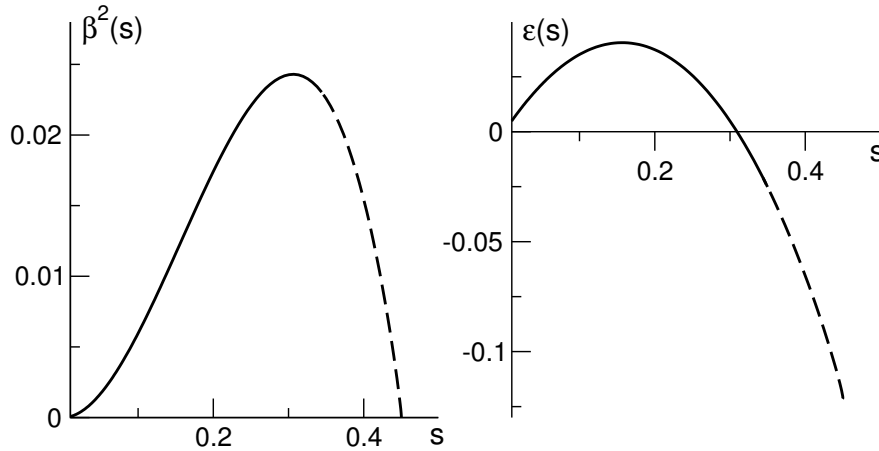
Fig. 4. Expansion factors \beta^2 and \epsilon plotted with respect to the control parameter s . The solid line part gives the parameter range of stable solutions V_0 , for which Turing instabilities might occur. The dashed line part denotes the parameter domain of unstable stationary solutions V_0 , cf. Fig. 2. In both panels a_e = 8 , a_i = 5.0 , and we applied the sigmoid function introduced in Fig. 1.
