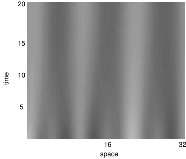
Fig. 12. Space-time plot revealing the Turing instability for local excitation-lateral inhibition interaction. Parameters are set to \xi_e = 1.0 , \xi_i = 2.0 , a_e = 6.0 , a_i = 5.0 with external stimulus I_0 = 2.36 yielding V_0 = 2.75 and s_c = 0.428 , k_c = 0.589 . The temporal evolution is calculated with dt = 0.01 while the space is discretized with dx = 0.08 , N = 400 . The greyscale encodes the deviation from the stationary state. The resulting pattern wavenumber agrees well with k_c .
