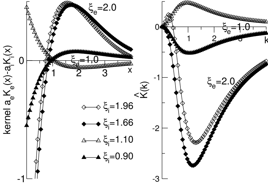
Fig. 10. The kernel function a_e K_e(x) - a_i K_i(x) and the function \hat{K}(k) for \xi_e \geq \xi_i . Parameter values are chosen according to Fig. 8. In case of \xi_e = 1.0 , local excitation-lateral inhibition ( \xi_i = 1.10 ) yields a local maximum of \hat{K} , i.e. Turing patterns, while local inhibition-lateral excitation ( \xi_i = 0.90 ) prohibits Turing patterns. In contrast, \xi_e = 2.0 exhibits local inhibition-lateral excitation for both values of \xi_i , while \hat{K} shows a local maximum for \xi_i = 1.96 . Here, a_e = 5, a_i = 5 .
