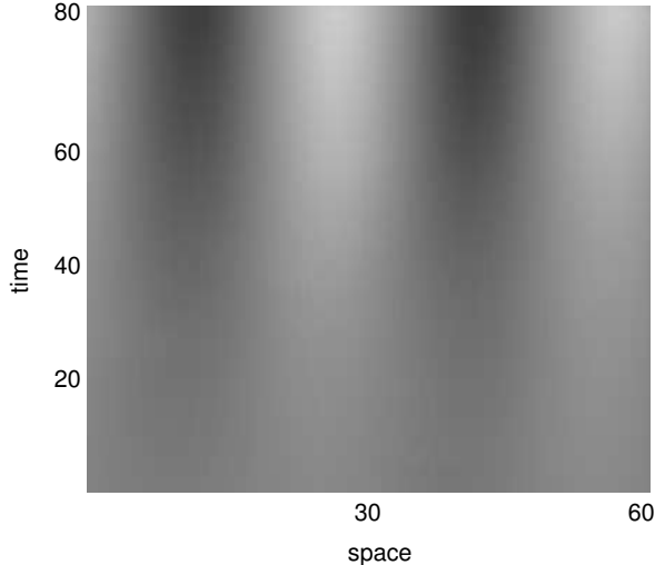
Fig. 13. Space-time plot revealing the Turing instability for local inhibition-lateral excitation interaction. Parameters are set to \xi_e = 2.0 , \xi_i = 1.92 , a_e = 131.0 , a_i = 130.0 with external stimulus I_0 = 2.2 yielding V_0 = 2.48 and s_c = 0.365 , k_c = 0.24 . The temporal evolution is calculated with dt = 0.01 while the space is discretized with dx = 0.15 , N = 400 . The greyscale encodes the deviation from the stationary state. The resulting pattern wavenumber agrees well with k_c .
