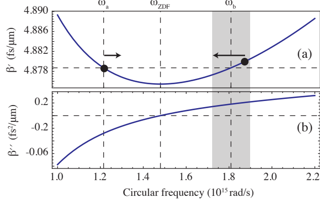
Figure 2: A typical profile (bulk silica) of (a) the group delay \beta'(\omega) and (b) GVD \beta''(\omega) that leads to the collision phenomenon shown in Fig. 1. Collision can only be realized for initial DW frequency offsets in a small interval (shaded gray) around the reference frequency of matching group velocity. Initial frequencies of soliton and DW are indicated by bullets, frequency shifts are indicated by arrows.
