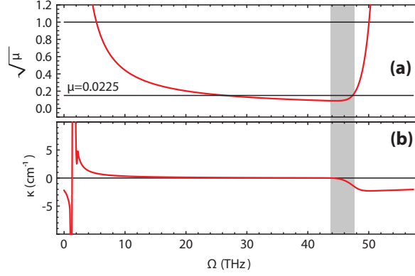
Figure 4: (a) Pairs of \Omega and relative DW amplitude \sqrt{\mu} for which solitons frequency does not change. Amplitude is plotted instead of power to facilitate readability. (b) Stability analysis. The region of stable SSFS compensation is shaded gray.
