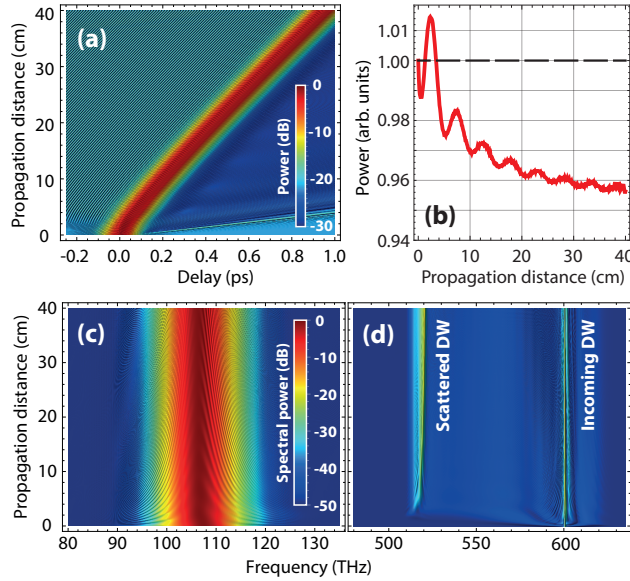
Figure 5: Compensation of SSFS by collision with a suitably prepared DW. (a) Evolution of soliton together with a DW in time domain as results from GNLSE. (b) Soliton amplitude is almost unchanged. (c) Soliton frequency is locked. (d) the scattered DW frequency is now well defined, cf., Fig 1(d). See Sec. 3 for parameters.
