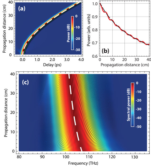
Figure 3: Space-time (a) and spectral (c) representation of a single soliton propagating along the fiber under influence of Raman effect from numerical simulation using full GNLSE. Additional dashed lines result from the adiabatic equations (7–9). (b) Soliton’s peak power from the GNLSE (red) and from the adiabatic equations (dashed). See Sec. 3 for parameters.
