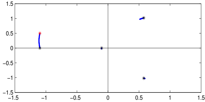
FIG. 7.2. Eigenvalue perturbation curves for the Hermitian pencil in Example 7.1 with respect to Hermitian perturbation.
