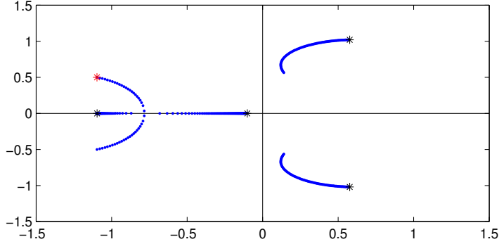
FIG. 7.1. Eigenvalue perturbation curves for the Hermitian pencil in Example 7.1 with respect to Hermitian perturbation.
