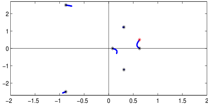
FIG. 7.6. Eigenvalue perturbation curves for the Hermitian polynomial Q(z) of Example 7.3 with respect to non Hermitian perturbation.
