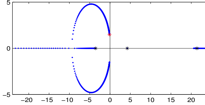
FIG. 7.3. Eigenvalue perturbation curves for the Hermitian pencil in Example 7.2 with respect to Hermitian perturbation.
