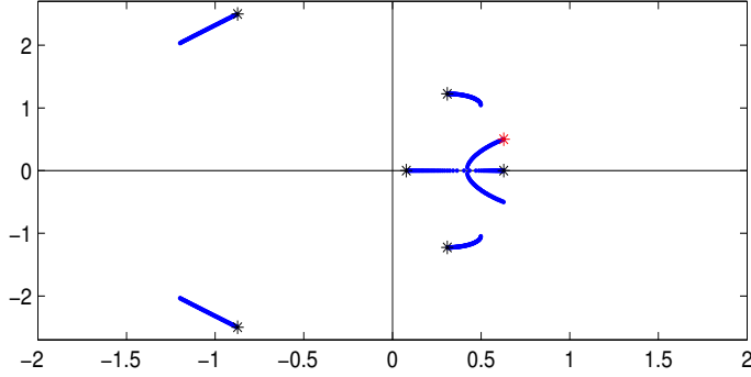
FIG. 7.5. Eigenvalue perturbation curves for the Hermitian polynomial Q(z) of Example 7.3 with respect to Hermitian perturbation.
