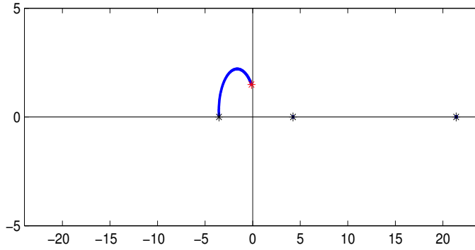
FIG. 7.4. Eigenvalue perturbation curves for the Hermitian pencil in Example 7.2 with respect to Hermitian perturbation.
