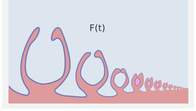
Figure 2: An example of a shrinking set where infinitely many exclusions during an "infinitesimal" time-interval have occurred.
