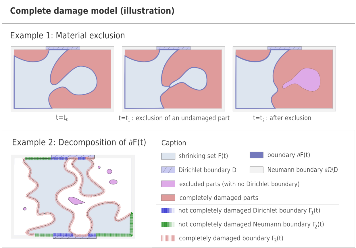
Figure 1: The first example in the illustration above shows the exclusion of an undamaged material part during the evolutionary process in 2D . The dark blue curve encircles the maximal admissible subset F(t) = \mathfrak{A}_D(\{z(t) > 0\}) of the not completely damaged area \{z(t) > 0\} . The second example below pictures the different parts of the boundary of F(t) . There, the Dirichlet boundary D consists of two components.
