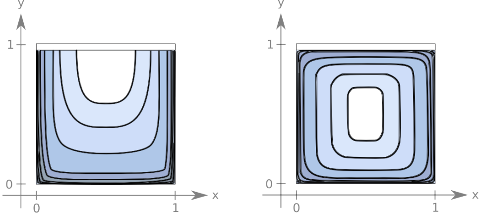
Figure 3: The left illustration shows a fine representation for the relatively open subset H = (0, 1) \times (0, 1] of \bar{\Omega} = [0, 1] \times [0, 1] whereas the right picture does not show a fine representation for H .
