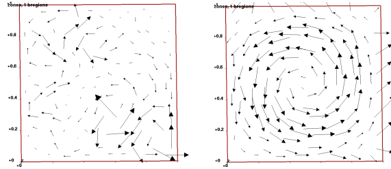
FIGURE 1. Numerical results on the mesh with mesh size \frac{1}{8} for the two finite volume schemes, \nu = 10^{-7} . Reconstructions of the discrete velocity are presented for the unmodified scheme (left) and for the scheme with divergence-free reconstruction (right)
