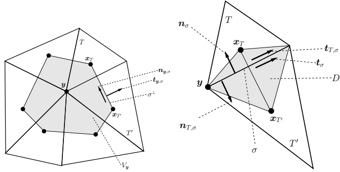
FIGURE 2. Notations for the mesh: Left: the Voronoi box associated to a vertex. Right: Zoom on a diamond.
