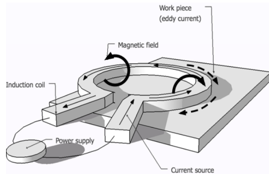
Figure 1: Illustration of electromagnetic induction heating.
