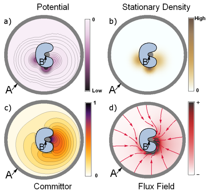
Figure 2: Illustration of TPT on a simple two-dimensional protein-ligand binding model. The dissociated state of the ligand A and the associated state B are shown. (a) potential energy landscape. (b) resulting stationary density, i.e., probability to find the ligand at a certain position (c) committor q , revealing a higher probability to reach the binding site for areas on top of the charged protein than for the uncharged protein. (d) reactive flux density and integrated flux lines calculated from the flux field resulting from the fluxes f_{ij}^+ .
