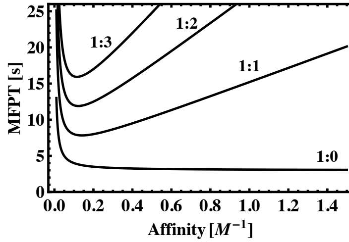
Figure 5: Mean binding time of a ligand in a mixture of “right” and “wrong” ligands at concentrations c_L and c_0 depending on the relative concentration c_L : c_0 and the pre-binding affinity K_a = k_{on}/k_{off} . Rates were set to (c_0 + c_L)k_{diff} = k_{AB} = k_{bind} = k_u = 1s^{-1} and k_{off} = k_{on}/K_a .
