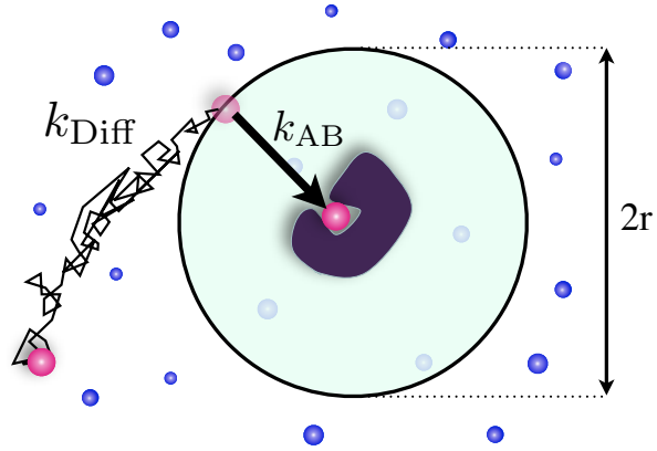
Figure 1: k_{\text{Diff}} and k_{\text{AB}} as contributors to the overall diffusional association rate k_{\text{on}} . k_{\text{Diff}} denotes the rate at which substrate particles diffuse into a sphere of radius r , it is given by the Smoluchowski rate k_{\text{Diff}} = 4\pi Dr and has the unit M^{-1}s^{-1} . k_{\text{AB}} denotes the transition rate of a single substrate molecule present at distance r to the binding site B , it is given by the A \rightarrow B transition rate and has the unit s^{-1} .
