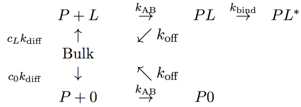
Figure 4: Reaction diagram showing a possible kinetic scenario of anion attraction to a pre-binding site. Starting from the bulk two possible reaction channels can be taken: In case of a ligand (L) the upper path is chosen, in case of a non-ligand (0) the lower one. Both species are attracted to the pre-binding site PL/P0 with their respective concentration dependent rate k_{on} , but only the ligand can move further to the bound state PL. If the concentration of non-ligand is increased with respect to the ligand concentration the lower channel will dominate the reaction system and the pre-binding site will be blocked by the non-ligand more often, which results in a lower yield of PL*.
