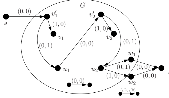
FIGURE 2.1. The values on the arcs show the cost assignments of the two scenarios S_1 and S_2 . The first-stage costs are set to 0.
