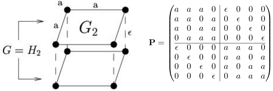
Figure 1: Left: G_2 is a bunkbed construction of the 2-dimensional hypercube H_2 . Right: if the weights on G_2 are chosen according to (10) the resulting stochastic matrix is \mathbf{P} with a = (1 - \epsilon)/3 .
