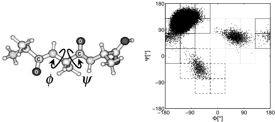
Figure 2: Left: The trialanine molecule shown in ball-and-stick representation. The overall structure of trialanine is primarily determined by the two torsion angles \Phi and \Psi . Right: Plotting \Phi versus \Psi results in a so-called Ramachandran plot. The discretization boxes are plotted with different edge lines indicating the different metastable sets they were allocated to.
