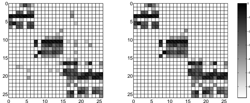
Figure 3: Left: The permuted transition matrix \mathbf{P} clearly has a block dominant structure. Right: In the resulting restricted matrix \mathbf{R} all off-diagonal entries are set to zero. The intensity of the boxes is chosen due to the logarithmic scale on the far right.
