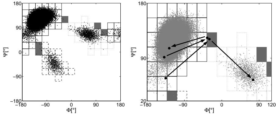
Figure 4: Left: A refined discretization produces boxes with large transition probabilities to other metastable sets. Here each torsion angle is discretized in 15 intervals. Boxes with a transition probability to another metastable set of 0.25 and larger are marked dark. Right: A close up illustrates the cause of this effect. The arrows connect subsequent sample points in the realization of the Markov chain.
