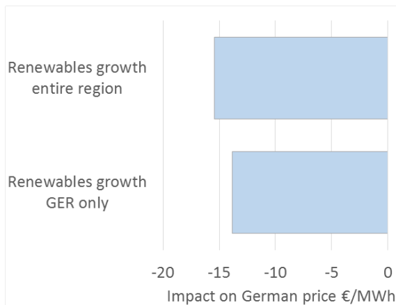
Figure 12. The impact of European vs. German renewable expansion on the German electricity price.
