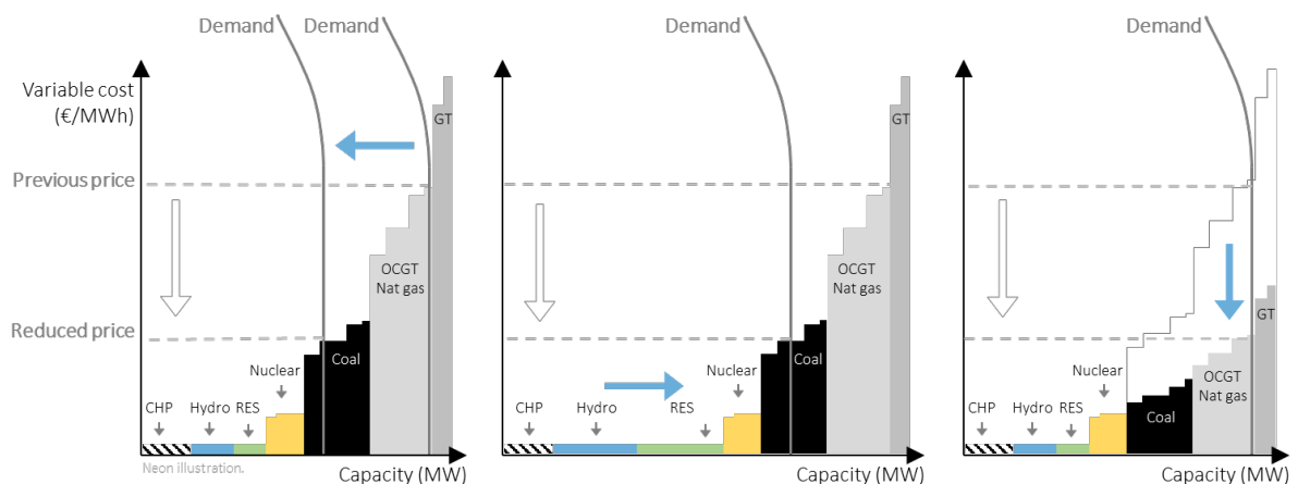
Figure 3. The impact of reduced electricity demand (left) is to shift the demand curve inwards. The impact of increased low-variable-cost supply (middle) is to shift the supply curve outward. The impact of reduced variable cost (right) is to shift the supply curve downward. Each shock (blue arrow) leads to a price decline (white arrow).
