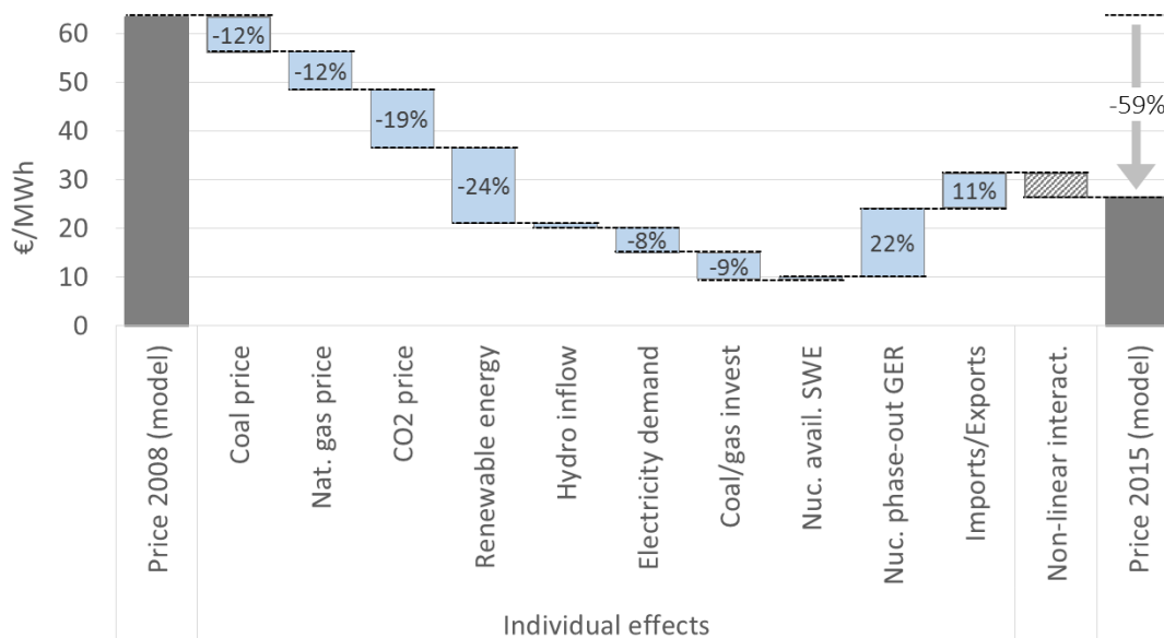
Figure 8. The change of German spot prices from 2008 to 2015 showing the contribution of ten individual factors. Numbers indicate the price impact of an individual factor relative to 2008 prices. For example, the effect of declining coal prices, holding everything else fixed, would have been a price decline of 12%. Overall, prices declined by 59%.
