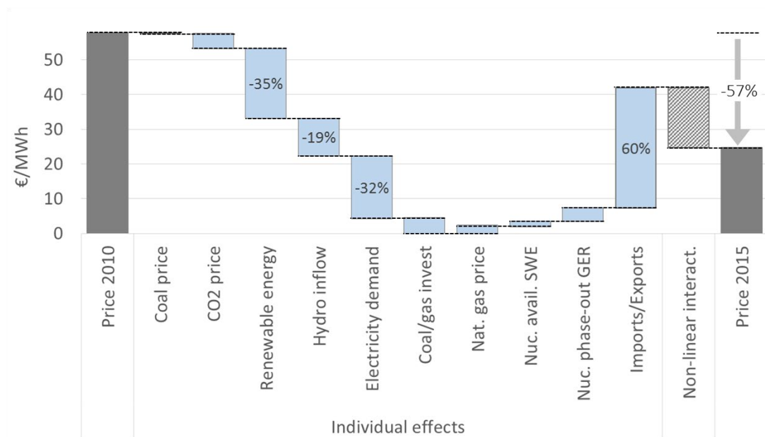
Figure 9. The change of Swedish spot prices from 2010 to 2015 showing the contribution of ten individual factors. Numbers indicate the price impact of an individual factor relative to 2010 prices.
