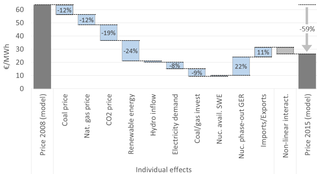
Graphical abstract – The change in German spot prices from 2008 to 2015, showing the contribution of ten individual drivers. Numbers indicate the price impact of an individual factor relative to 2008 prices. For example, the decline of coal prices on its own would have caused an electricity price drop of 12%. In contrast, the nuclear phase-out alone would have increased prices by 22% from 2008 levels. Overall, electricity prices fell by 59%.
