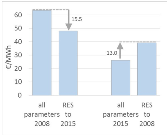
Figure 10. Germany: the impact of renewable energy for different reference years.
