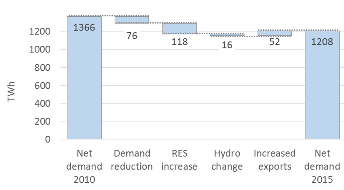
Figure 4. The change in model-region net demand (demand to be served from thermal power plants) from 2010 to 2015.
