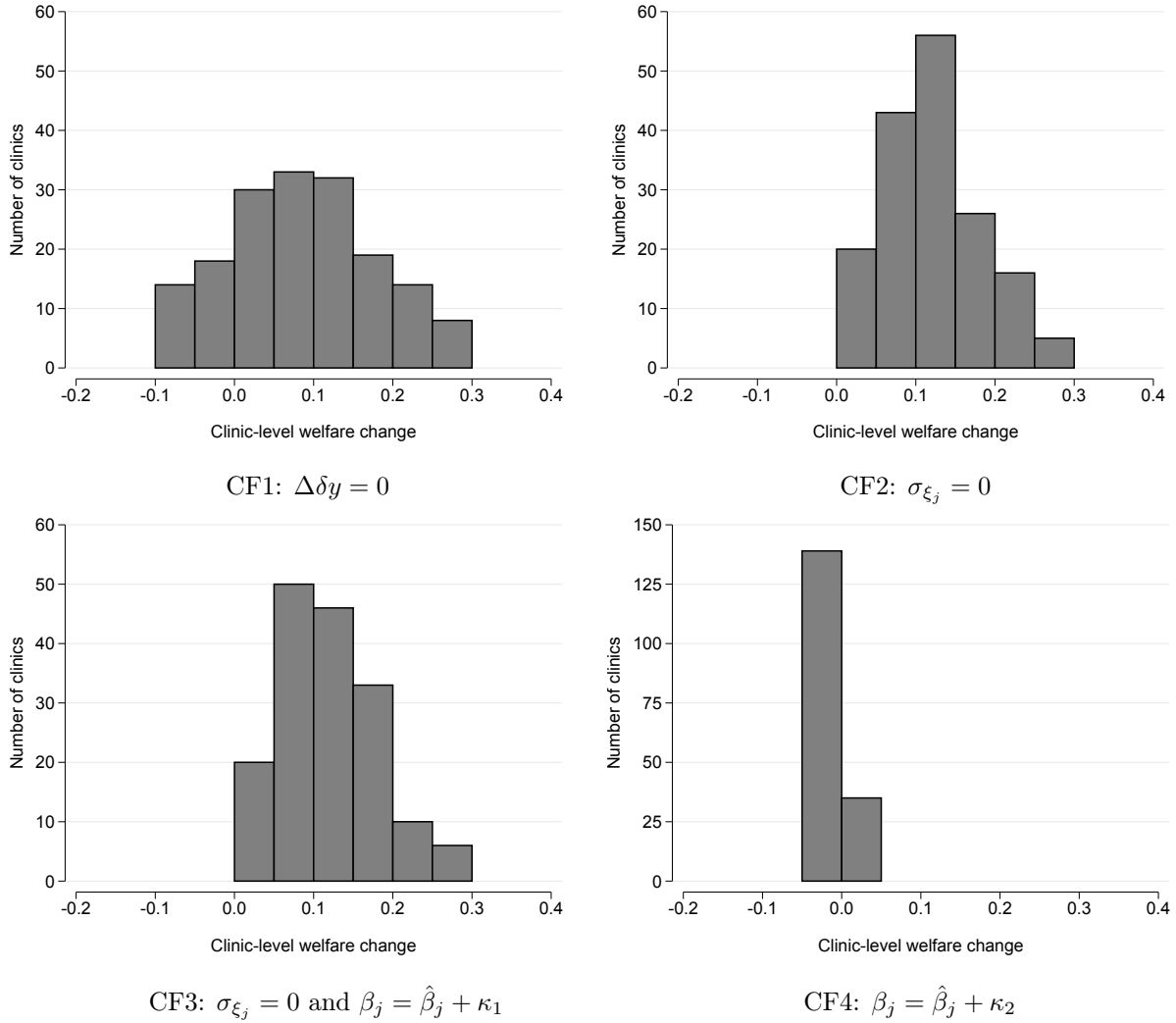
Figure 2: Distribution of counterfactual payoff changes, W_j
