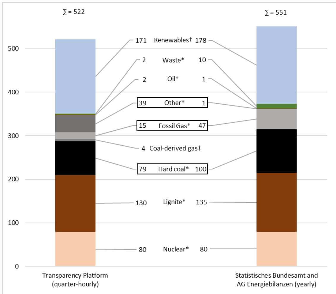
Figure 6. Comparing “Aggregated Generation per Type” (16.1.B&C) with 2016 German generation data from Destatis and AG Energiebilanzen. TP reports noticeably smaller values for fossil gas and hard coal compared to other sources. *yearly data from Destatis, †yearly data from AG Energiebilanzen, ‡no equivalent in Destatis/AG Energiebilanzen.
