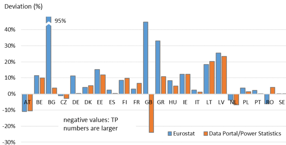
Figure 8. Deviation of wind generation between TP and other sources. TP wind generation data (16.1.C) often deviate significantly from other sources (>10%), including ENTSO-E Power Statistics.
