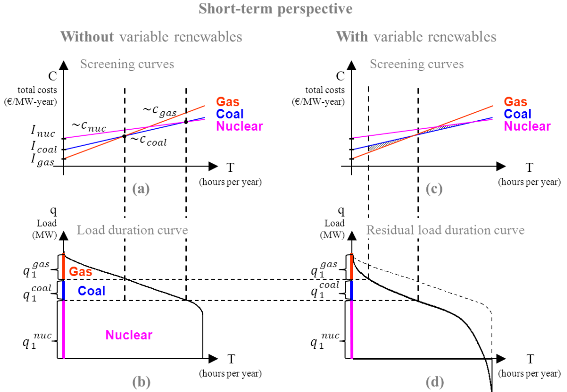
Figure 8 (illustrative): Optimal long-term capacities are derived without VRE (a, b). With VRE the LDC transforms to a RLDC (d). In the short-term perspective the capacities remain unchanged (b, d). Hence, specific costs increase because technologies operate in full-load hour ranges where they would not be cost-efficient if capacities could optimally adjust (c).
