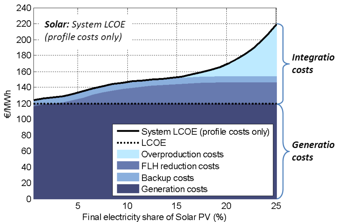
Figure 10: System LCOE (profile costs only) for increasing generation shares of wind (above) and solar PV (below) for Germany estimated with a power system model that is designed for calculating profile costs. These costs are decomposed into three cost drivers. The full-load hour (FLH) reduction of conventional plants is the largest cost driver at moderate shares, while overproduction costs significantly increase integration costs at high shares.
