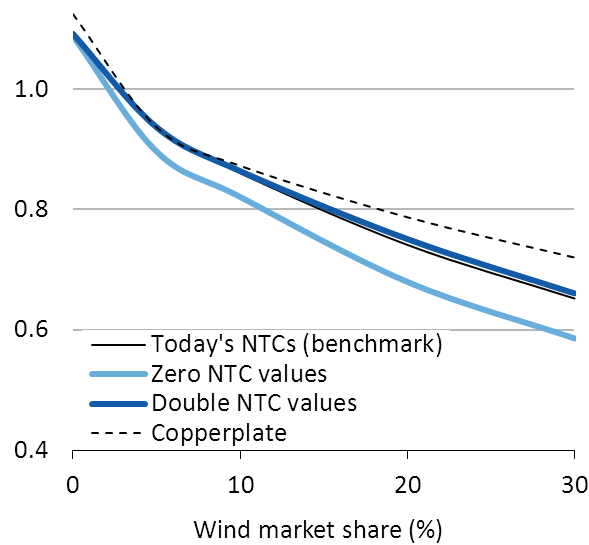
Figure 24. Long-term wind value factors in the model region at different NTC assumptions. The impact of doubling NTC capacity is moderate in size, but positive in all countries.
