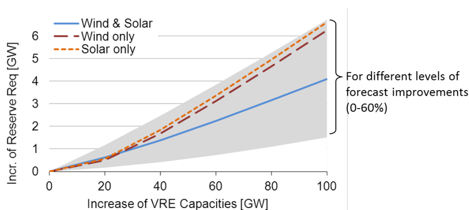
Figure 6. The impact of additional VRE capacity on balancing reserve requirement as estimated by Ziegenhagen (2013).
