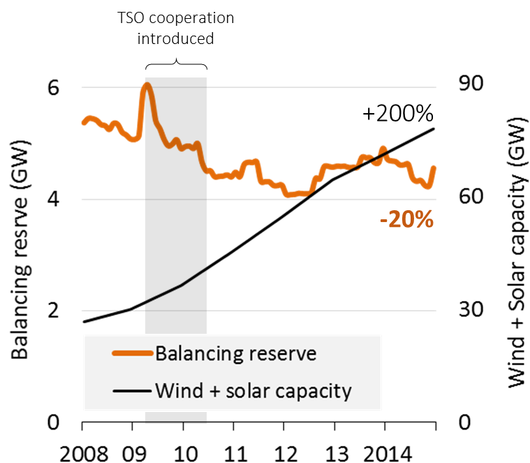
Figure 7. Balancing reserves (SC + TC, average of positive and negative reserve) and VRE capacity (wind + solar) in Germany. Even though the installed capacity of wind and solar power has tripled since 2008, the demand for balancing power has decreased. One reason was the cooperation between TSOs introduced in 2009/10.
