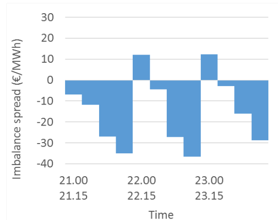
Figure 20. The quarter-hourly imbalance spread during the evening ramp. Just before the full hour, the system is long, leading to negative spreads.
