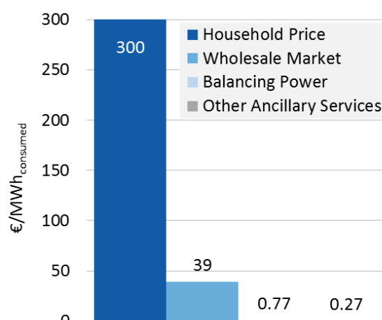
Figure 9. The cost of balancing power provision is very small when compared to the wholesale market for energy or the retail prices. Source: own calculations, Bundesnetzagentur (2014).
