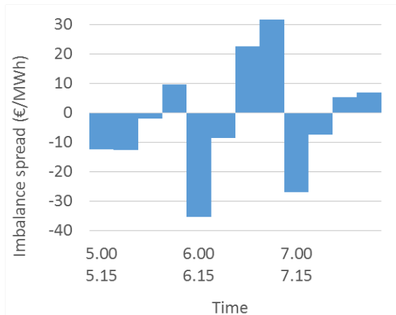
Figure 19. The quarter-hourly imbalance spread during the morning ramp. Just before the full hour, the system is short, leading to positive spreads.
