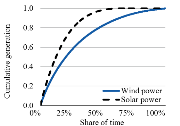
Figure 9. Cumulative distribution functions of solar and wind power. Solar is more concentrated than wind.
