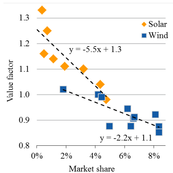
Figure 4. Historical wind and solar value factors in Germany from spot prices (reflecting profile costs). As solar penetration increased from zero to 4.7%, its value factor decreased from 1.33 to 0.98.
