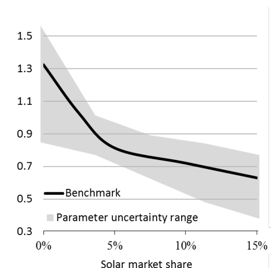
Figure 14. Long-term solar value factor drops to 0.4 – 0.8 at 15% penetration rate.
