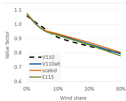
Figure 10. Comparing V110 to alternative advanced profiles. All profiles show a very similar pattern.
