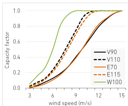
Figure 21. The power curve of a hypothetical “super advanced” turbine with a specific rating of roughly 100 W/m 2 .
