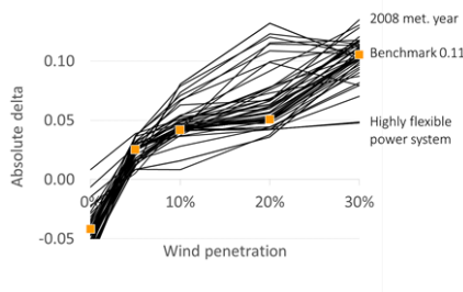
Figure 13. The delta between classical and advanced turbines is remarkably robust: at 30% penetration, 95% of all sensitivities fall between 8.5 and 14.5 percentage points.
