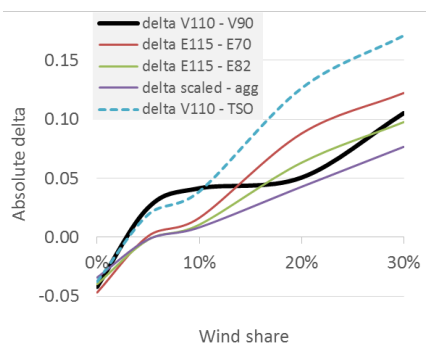
Figure 11. Alternative pairs of profiles to determine the market value delta between classical and advanced turbines.
