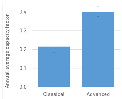
Figure 3. Annual average capacity factors, as derived from these power curves, using data from the weather year 2009 in Germany. Error bars show variation 2008-12. The classical capacity factor of 0.21 corresponds to 1880 full load hours (FLH), the advanced capacity factor of 0.4 to 3500 FLH.
