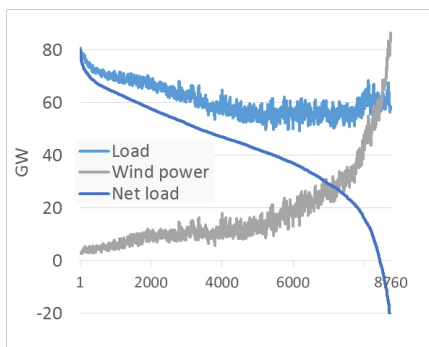
Figure 25. 30% wind with classical technology. Low net (residual) load levels become wind dominated, load levels are actually quite high during some times at low net load
