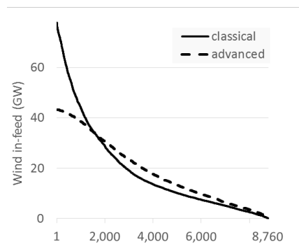
Figure 5. In-feed duration curves (ordered hourly generation) for classical and advanced turbines in Germany, assuming a wind penetration rate of 30%. Annual energy output is the same for both lines, installed capacities differ.
