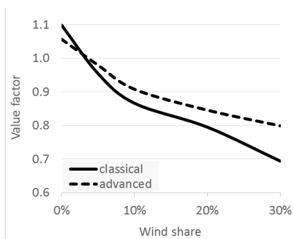
Figure 6. The gap between the black line (classical) and the black dotted line (advanced) represents the impact of advanced turbine technology. The gap is 11 percentage points at 30% penetration.
