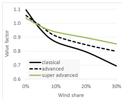
Figure 22. The market value of a “super advanced” turbine with a specific power rating of 100 W/m 2 is not much higher than that of advanced design.
