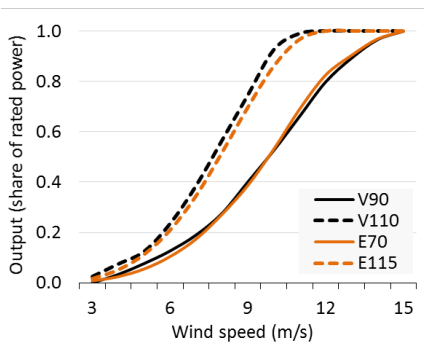
Figure 8. Alternative power curves used for sensitivity analyses.
