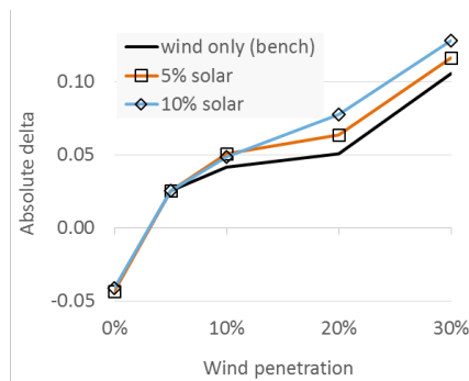
Figure 16. Wind deltas for different solar penetration rates. If solar power is added, the delta increases.
