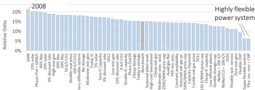
Figure 14. Relative delta at 30% penetration. In 95% of all sensitivity runs, the relative delta is in the range of 10 – 20%.
