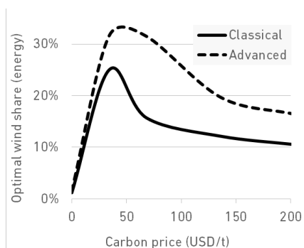
Figure 20. Optimal share of wind power as a function of the CO 2 price. Advanced turbines have a 50% higher optimal deployment level (assuming identical LEC).
