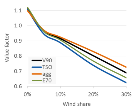
Figure 9. Comparing V90 to alternative classical profiles. All profiles show a similar pattern, two out of three are below V90.
