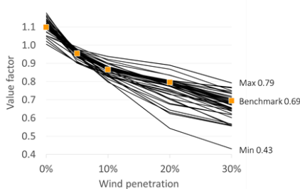
Figure 12. The value factor of classical turbines in all sensitivities. Parameter uncertainty leads to a quite broad range of estimates at high penetration.
