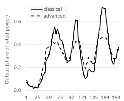
Figure 4. Chronological in-feed during ten days. Annual energy output is the same for both lines, installed capacities differ.
