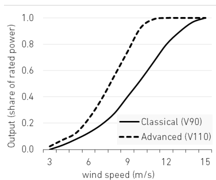
Figure 2. Power curves of a "classical" (Vestas V90) and an "advanced" turbine (Vestas V110).
