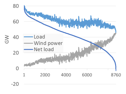
Figure 26. 30% wind with advanced technology. Net load remains more load driven
