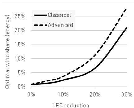
Figure 19. Optimal share of wind power in energy terms as a function of wind LEC reductions relative to today. Classical and advanced wind turbines are assumed to have the same LEC. The model assumption translate to LEC of USD 75 per MWh (0% reduction), which translates to USD 53 at 30% reduction.
