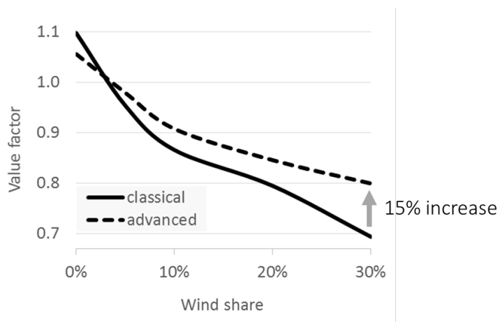
Graphical abstract – The market value of wind power as a function of wind penetration in annual energy terms. Value is expressed relative to the average electricity price (value factor). At 30% market share, each MWh of wind power is worth 15% more if generated by advanced turbines compared to classical technology.
