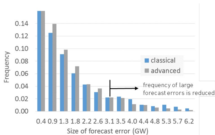
Figure 23. Distribution of one-hour persistence forecast errors (at 30% wind penetration, corresponding to 90 GW classical wind capacity). With advanced turbines, large forecast errors (above 3.1 GW) occur less frequently.
