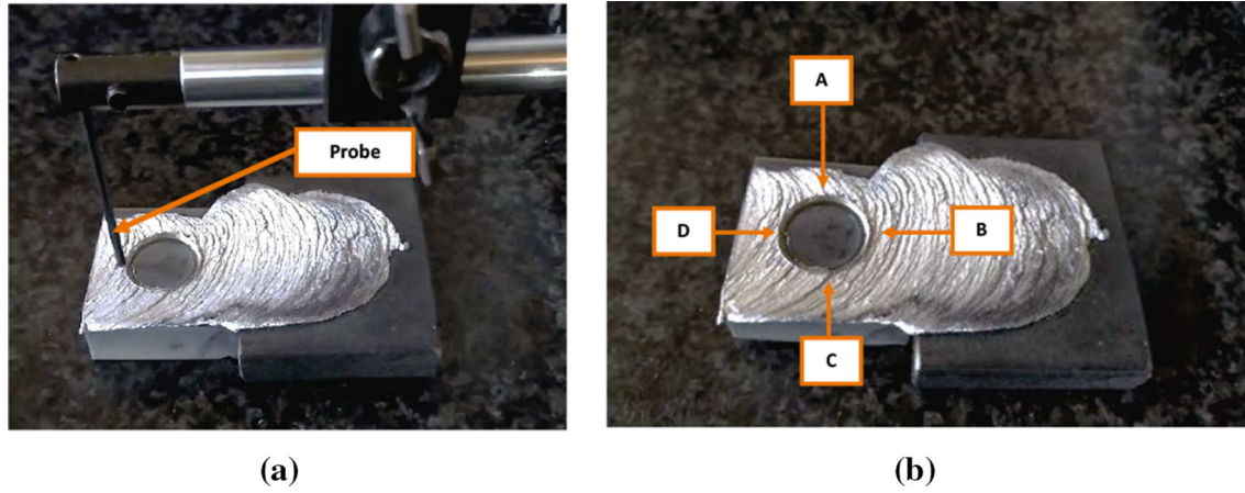
Fig. 6—Measuring instrument showing (a) probe and (b) coating thickness measurement points.
