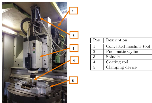
Fig. 2—Machine set-up.
