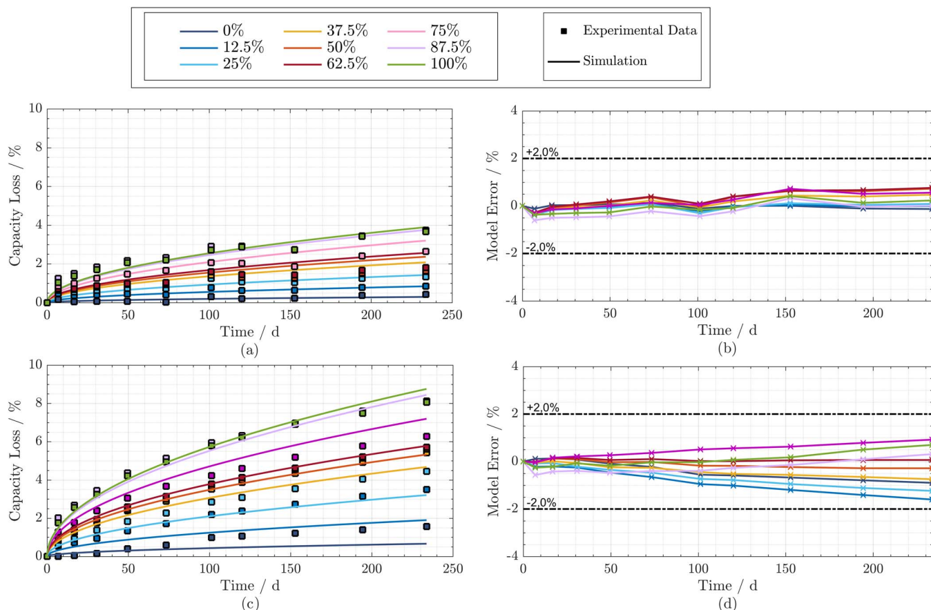
Figure 12. Comparison of model and experimental data for storage tests: a) Capacity loss at T = 15^{\circ}C , b) Model error at T = 15^{\circ}C , c) Capacity loss at T = 45^{\circ}C , d) Model error at T = 45^{\circ}C .
