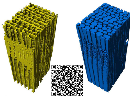
Fig. 3 Visualization of cell wall (yellow, left) and lumina (blue, right) volumes of representative 3D areas of spruce's early wood region. ROI: 0.13 mm 2 . For 3D animation please follow QR code.
