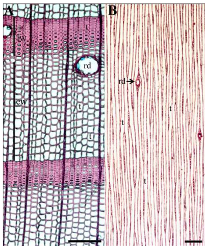
Fig. 1 Light microscopy images of spruce wood. A: cross section; B: tangential section through early wood region, ew-early wood; lw-late wood; rd- resin duct; t-tracheid. Scale bars represent 200 \mu m
