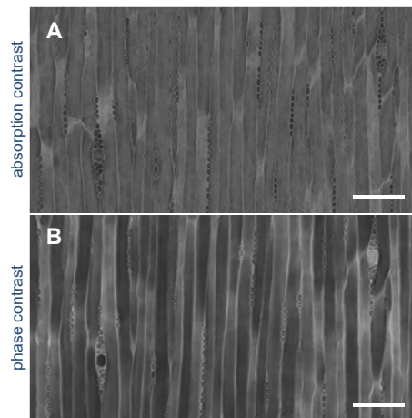
Fig. 2 Horizontal slice through tomographic reconstructions where flat-and-dark field corrected projections (A) or retrieved phase maps (B) served as input. Scale bars represent 200 \mu m
