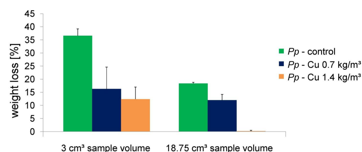
Figure 2: Weight loss after six weeks from different volume samples of Pinus sylvestris L. treated with two different concentrations of copper sulphate ( \text{CuSO}_4 \cdot 5 \text{H}_2\text{O} ) [1] Pp - Poria placenta ; n = 4
