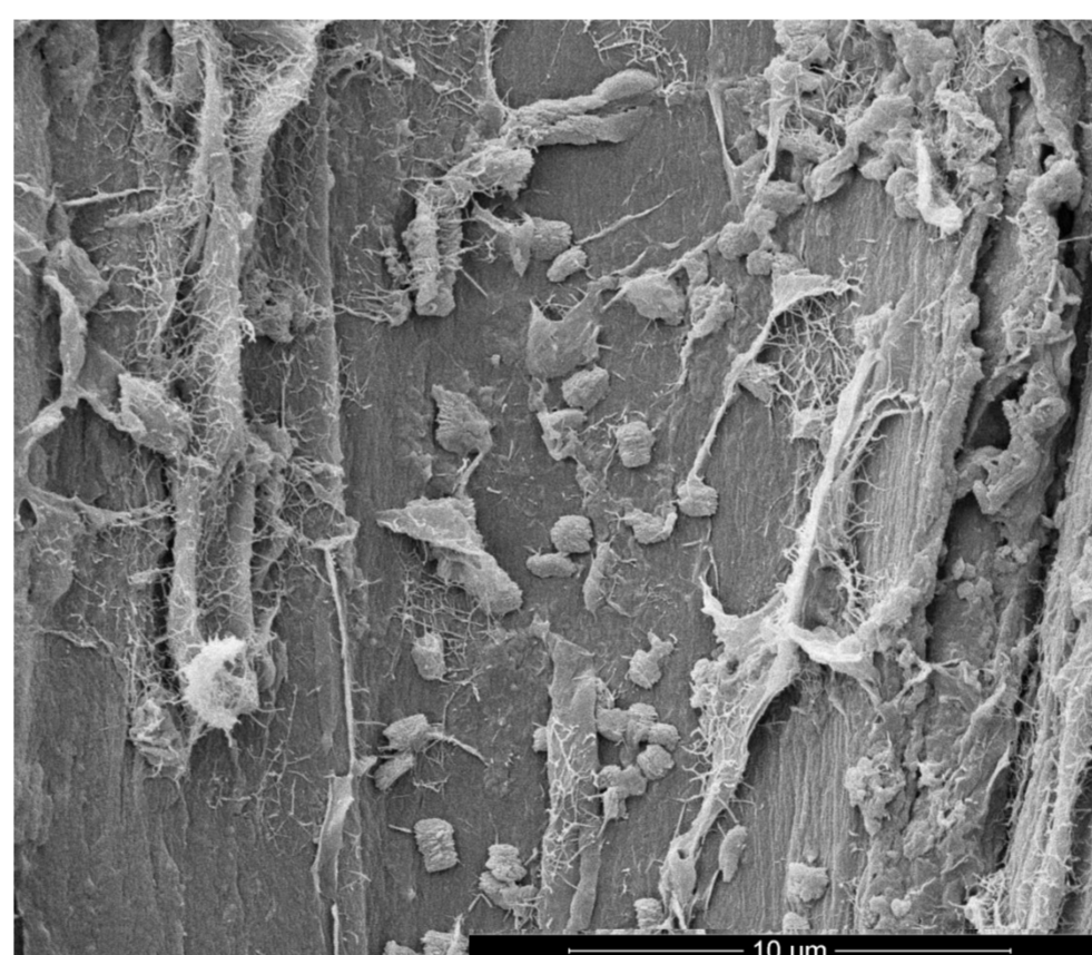
Figure 4: Surface of Pinus sylvestris L. containing 0.7 kg/m 3 of copper. Copper oxalate crystals of different sizes were found.
