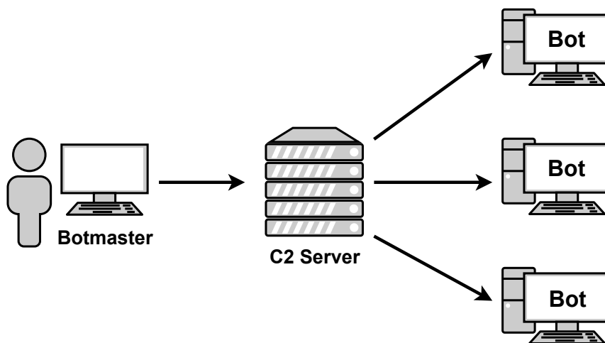
Figure 2.2.: Botnet [9]
