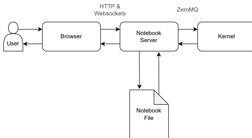
Figure 2.1.: Jupyter Notebook [6]
