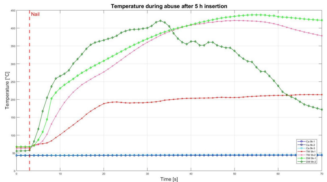
Figure 10. Temperatures during nail penetration test for all cells of category 5 h insertion in different insertion media: CaCl 2 (blue), TW (red) and DW (green), maximum temperature difference: Ca 5h-1 = 0.7 °C; Ca 5h-2 = 0.5 °C; Ca 5h-3 = 0.6 °C; TW 5h-1 = 150.2 °C; TW 5h-2 = 358.8 °C; DW 5h-1 = 370 °C; DW 5h-2 = 363.3 °C.
