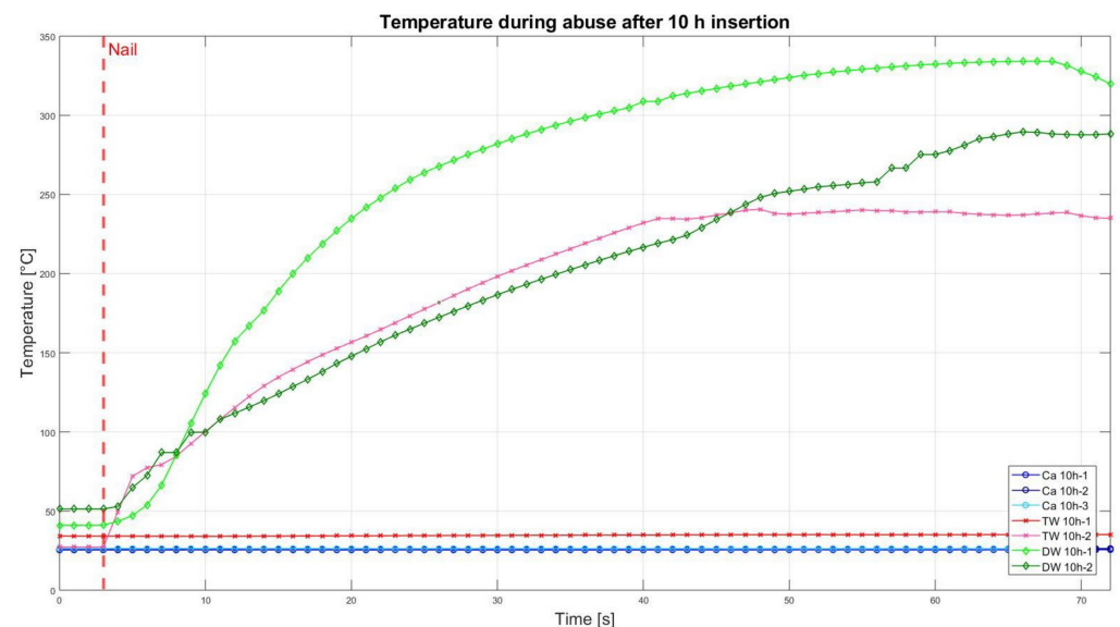
Figure 11. Temperatures during nail penetration test for all cells of category 10 h insertion in different insertion media: CaCl 2 (blue), TW (red) and DW (green), maximum temperature difference: Ca 10h-1 = 0.1 °C; Ca 10h-2 = 1.4 °C; Ca 10h-3 = 0.2 °C; TW 10h-1 = 0.3 °C; TW 10h-2 = 213.5 °C; DW 10h-1 = 293 °C; DW 10h-2 = 238.3 °C.
