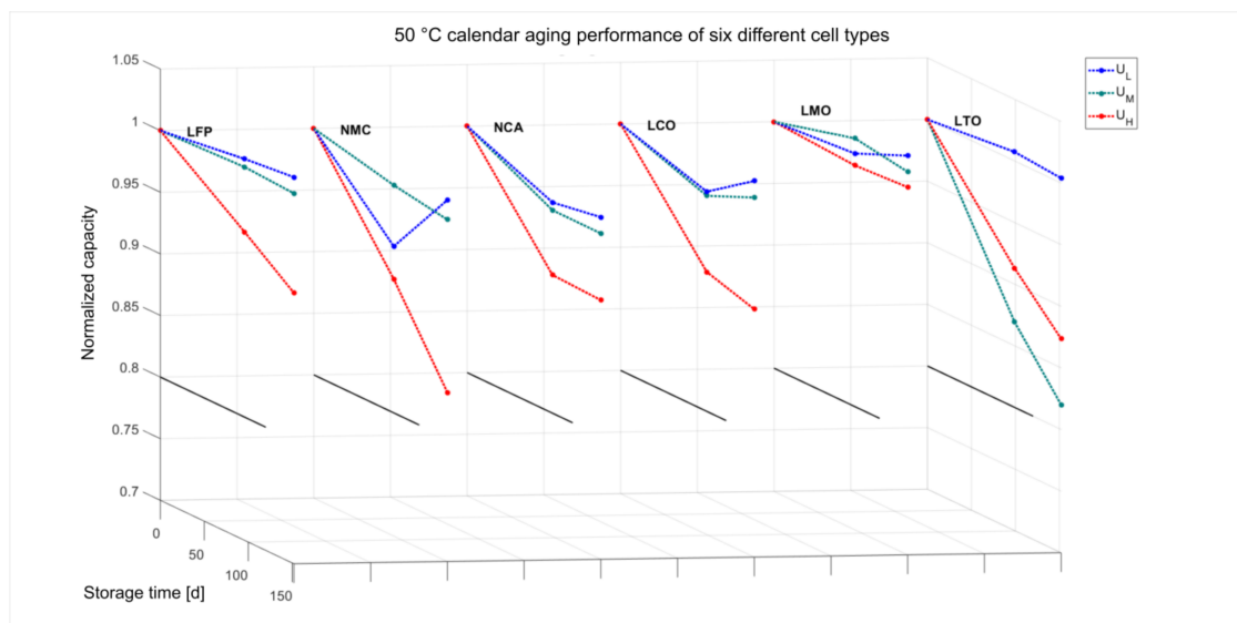
Figure 4. Normalized discharge-capacity decrease of six chemistries at 50^\circ\text{C} storage over 150 days at three storage voltages ( U_L -voltage low, U_M -voltage mid, U_H -voltage high), each plotted point displays the average capacity of all individual cells at that same condition.
