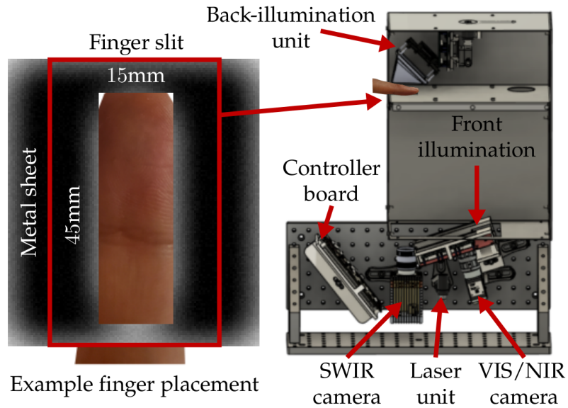
Figure a.4: Fingerprint capture device (version 2) as illustrated in [268]. The InGaAs camera was replaced and only one lens is used now. Hence, the lens flipper and mirror could also be removed. Additional technicals details are included in [267].
