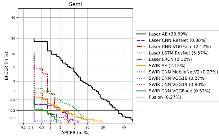
Figure 3.53: DET curves of the Semi transparent group and their corresponding APCER_{0.2} values.
