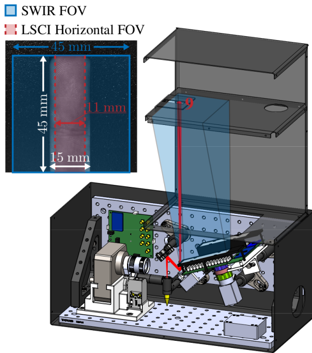
(b) Field of view (FOV) and light paths.
