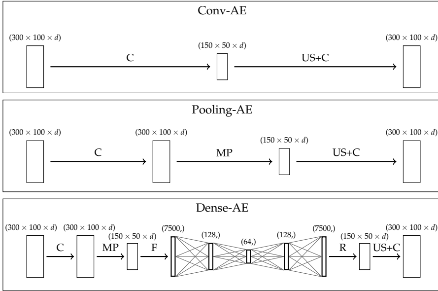
Figure 3.36: Autoencoder architectures for variable image dimensions d . The following operations are used: C = convolution, US = up-sampling, MP = max pooling, F = flatten, R = reshape.
