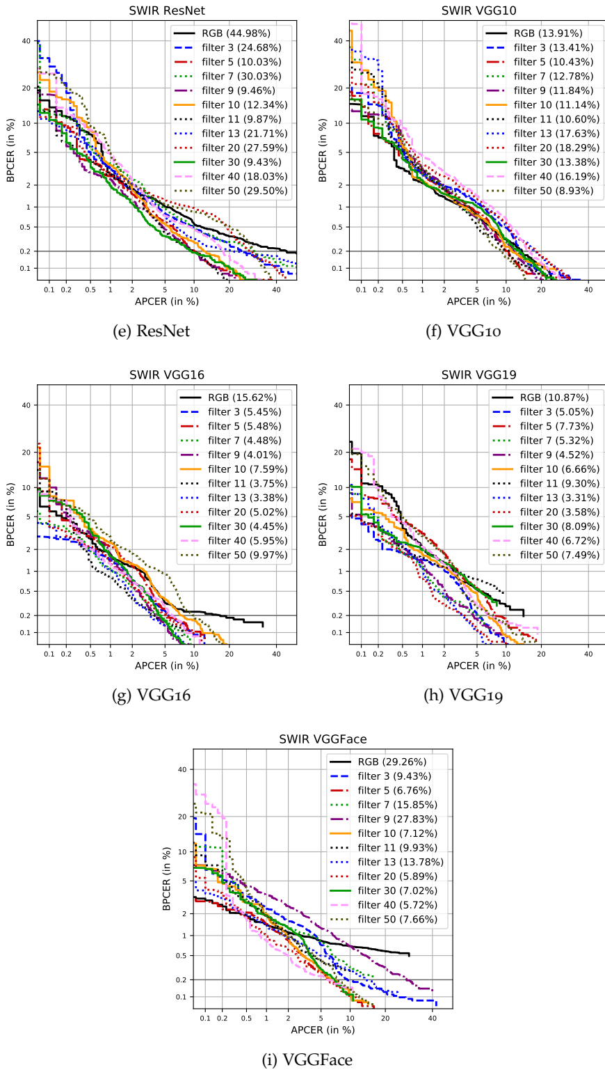
Figure 3.41: SWIR benchmark results (2/2). APCER_{0.2} values are given in brackets.
