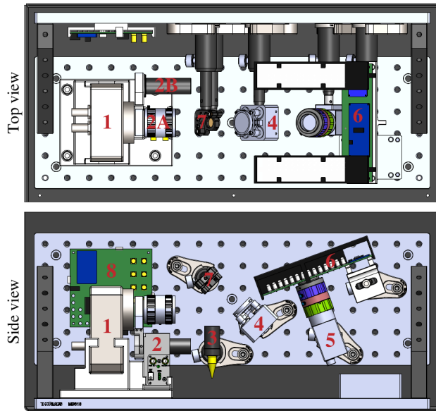
(a) Lower compartment of the capture device.
