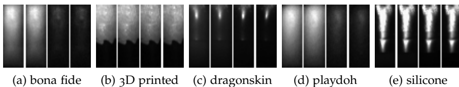
Figure 3.5: SWIR samples in the four wavelengths 1200, 1300, 1450, 1550 nm.
