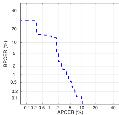
Figure 3.28: DET curve of Fusion I on the handcrafted partition.
