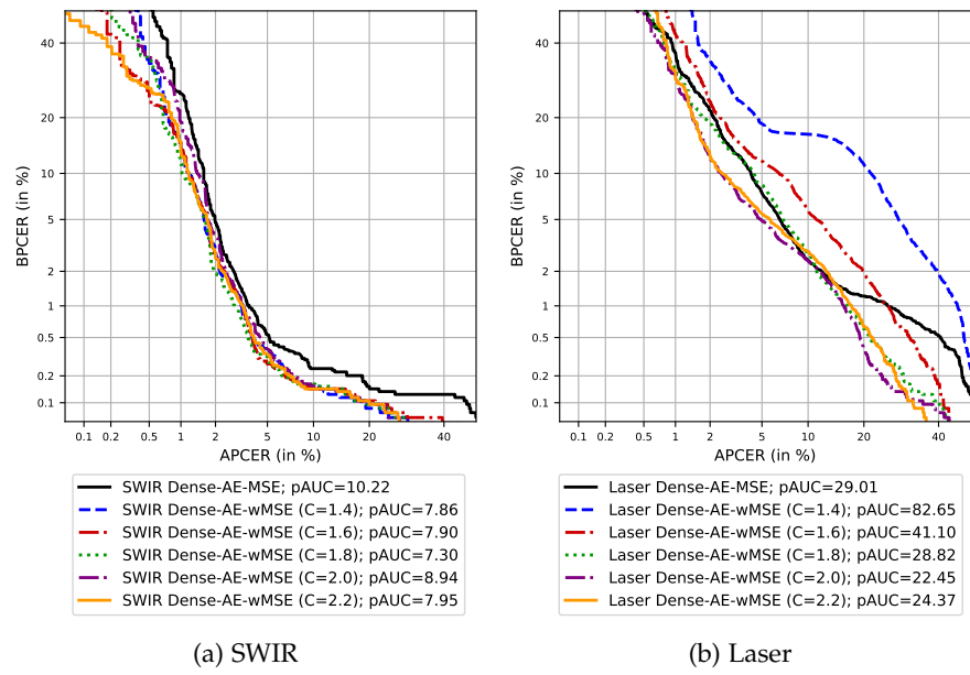
Figure 3.45: Performance of the Dense-AEs on SWIR and laser data for MSE and wMSE settings. The pAUC is given in %.
