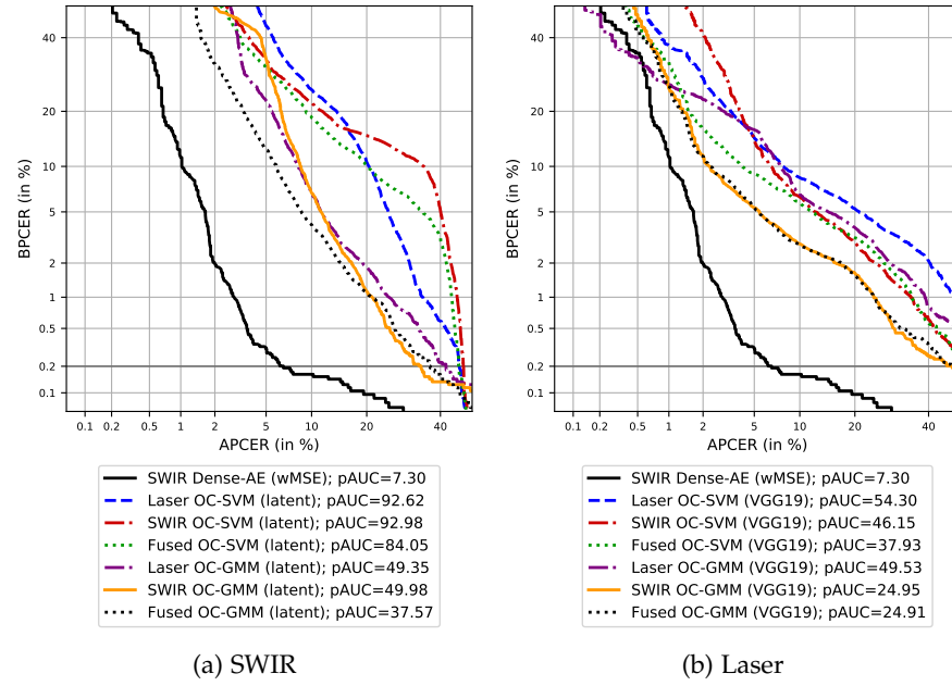
Figure 3.47: Benchmark of the best AE setup towards additional OC classifiers based on two different features.
