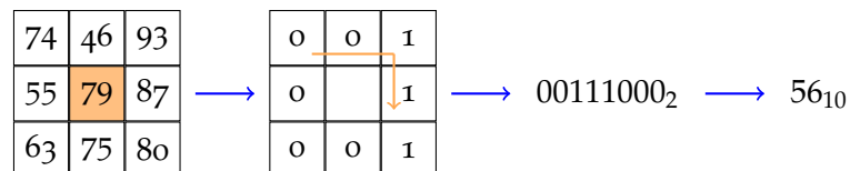
Figure 3.11: LBP computation steps for a 3 \times 3 window.
