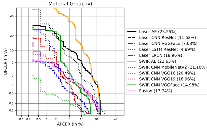
Figure 3.57: DET curves of the material group iv) and their corresponding APCER_{0.2} values.
