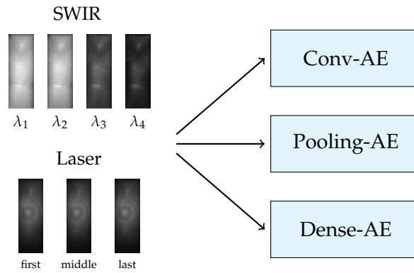
Figure 3.39: Structure of the AE PAD approaches.
