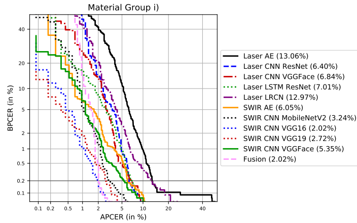
Figure 3.54: DET curves of the material group i) and their corresponding APCER_{0.2} values.
