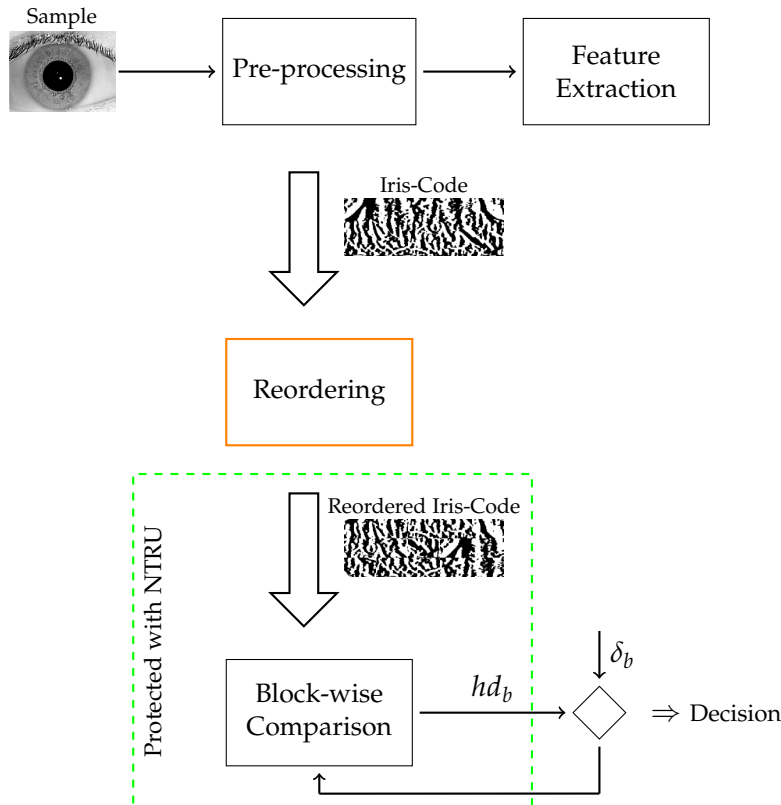
Figure 4.5: The ordinary iris-code is extracted from the pre-processed sample. The proposed modifications consists of reordering, encryption, and a block-wise comparison to accelerate the process.
