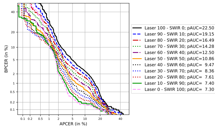
Figure 3.46: Weighted score fusions of the best-performing wMSE Dense-AEs. The pAUC is given in %.
