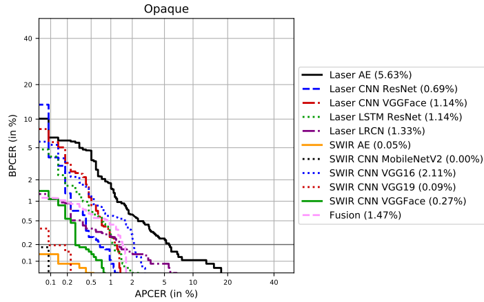
Figure 3.51: DET curves of the Opaque group and their corresponding APCER_{0.2} values.
