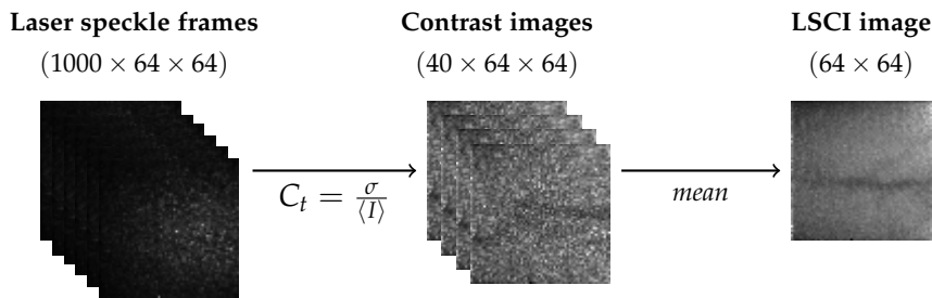
Figure 3.8: LSCI pre-processing pipeline computing the temporal contrast of the captured laser speckle sequence.
