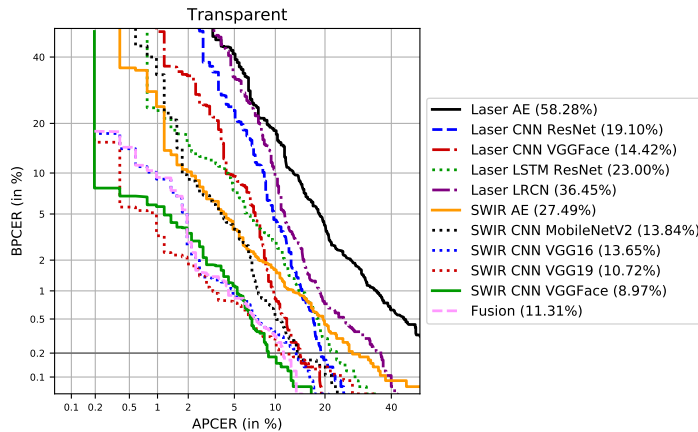
Figure 3.52: DET curves of the Transparent group and their corresponding APCER_{0.2} values.
