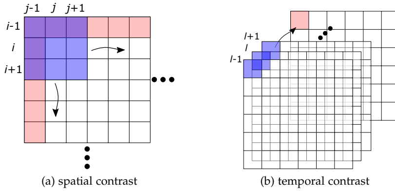
Figure 3.7: Laser speckle contrast calculation for (a) spatial and (b) temporal domain as described in [288].
