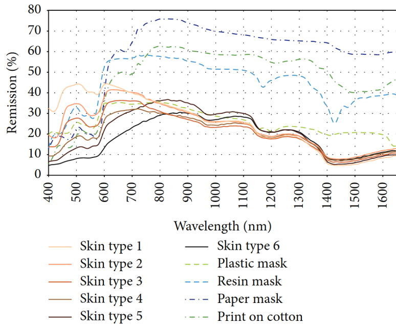
Figure a.3: Spectral remission intensities of skin and different PAI materials as illustrated in [271]. The SWIR spectrum is in the range of 1200 nm to 1700 nm, which is the area where different skin types align.
