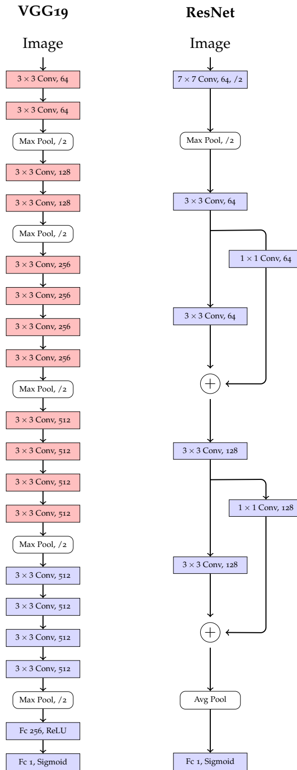
Figure 3.14: CNN architectures of the fine-tuned VGG19 and the developed residual CNN ResNet. Trainable layers are coloured in blue and red marks pre-trained layers that keep original weights.
