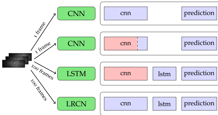
Figure 3.38: Structure of the laser PAD approaches with trainable blocks coloured in blue and fixed ones are marked in red.
