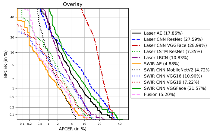
Figure 3.50: DET curves of the Overlay group and their corresponding APCER_{0.2} values.
