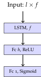
Figure 3.34: LSTM architecture based on sequence length l and extracted feature vector size f = 4 \times h . The LSTM layer processes the sequence but preserve the feature length, the first fully connected layer reduces the vector by a factor of four, and the final fully connected layer outputs a PAD score between 0 and 1.
