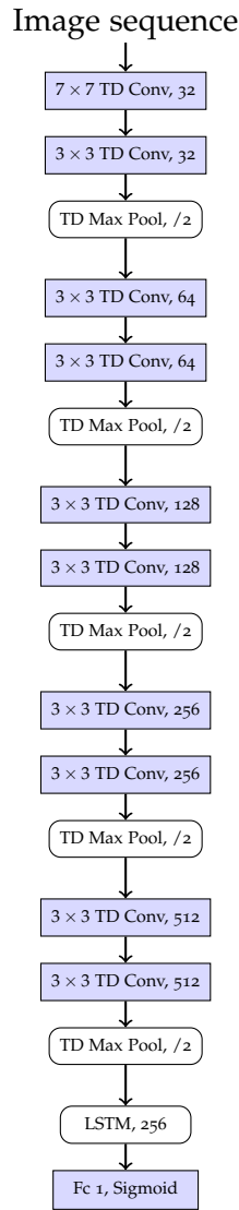
Figure 3.35: LRCN architecture. All layers, except LSTM and fully connected, are time distributed (TD) and all blocks are trained from scratch.
