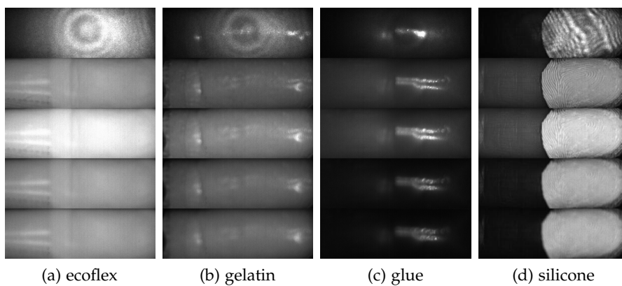
Figure 3.31: Samples of four different PAIs across all five wavelengths. Top to bottom: 1310 nm laser, 1200 nm, 1300 nm, 1450 nm, and 1550 nm SWIR.
