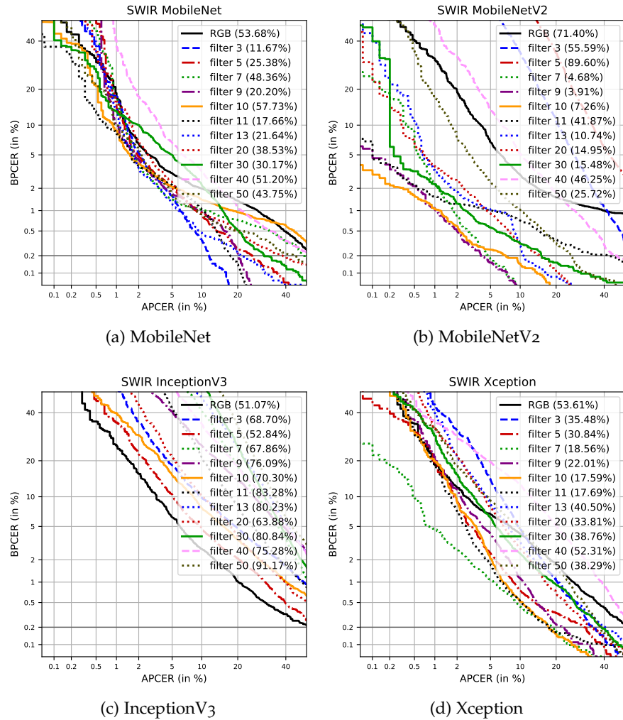
Figure 3.41: SWIR benchmark results (1/2). APCER_{0.2} values are given in brackets.
