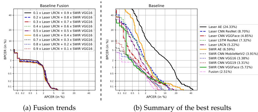
Figure 3.48: Overview of different weighted fusions (a) and the best PAD algorithms with their corresponding APCER_{0.2} values (b).
