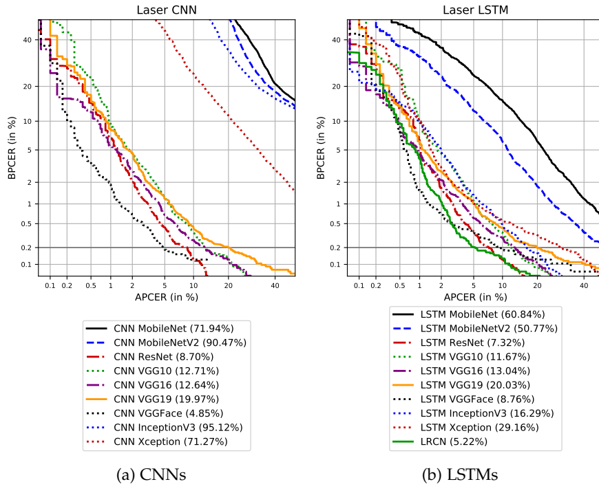
Figure 3.43: Laser benchmark results. APCER_{0.2} values are given in brackets.
