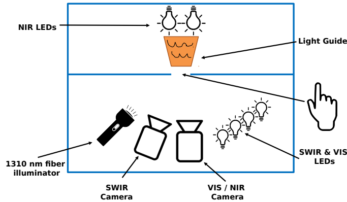
Figure 3.1: The capture device is a closed box with only one free slot for the finger. Two cameras in combination with multiple illuminations are able to capture the fingerprint and additional PAD data.
