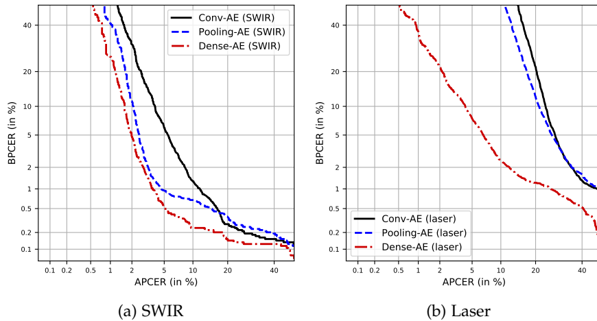
Figure 3.44: DET curves for the three baseline AE architectures: Conv-AE, Pooling-AE, and Dense-AE.
