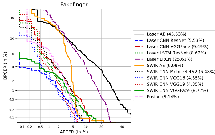
Figure 3.49: DET curves of the Fakefinger group and their corresponding APCER 0.2 values.
