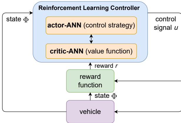
Fig. 5. Principle of Reinforcement Learning
