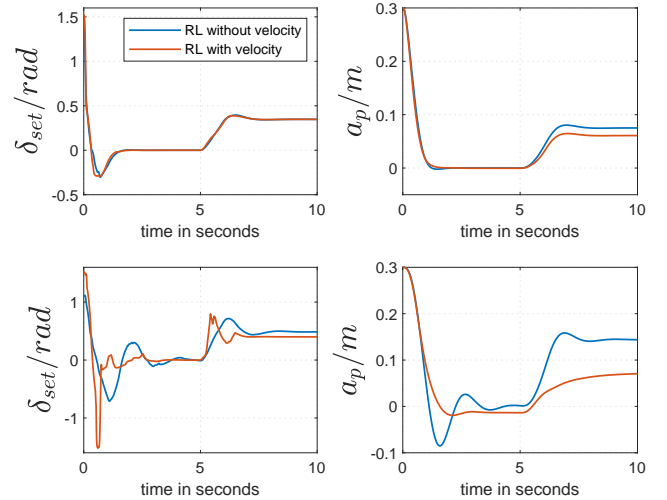
Fig. 11. Steering angle and lateral deviation of Linde E30 (top) and Linde E80 (bottom) for v = 2\text{m/s}
