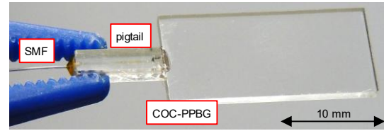
Fig. 2: COC-PPBG butt-coupled to a pigtailed standard single-mode fiber.
