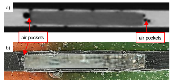
Fig. 6: a) CT scan and b) microsection of CFRP-integrated PPBG.
