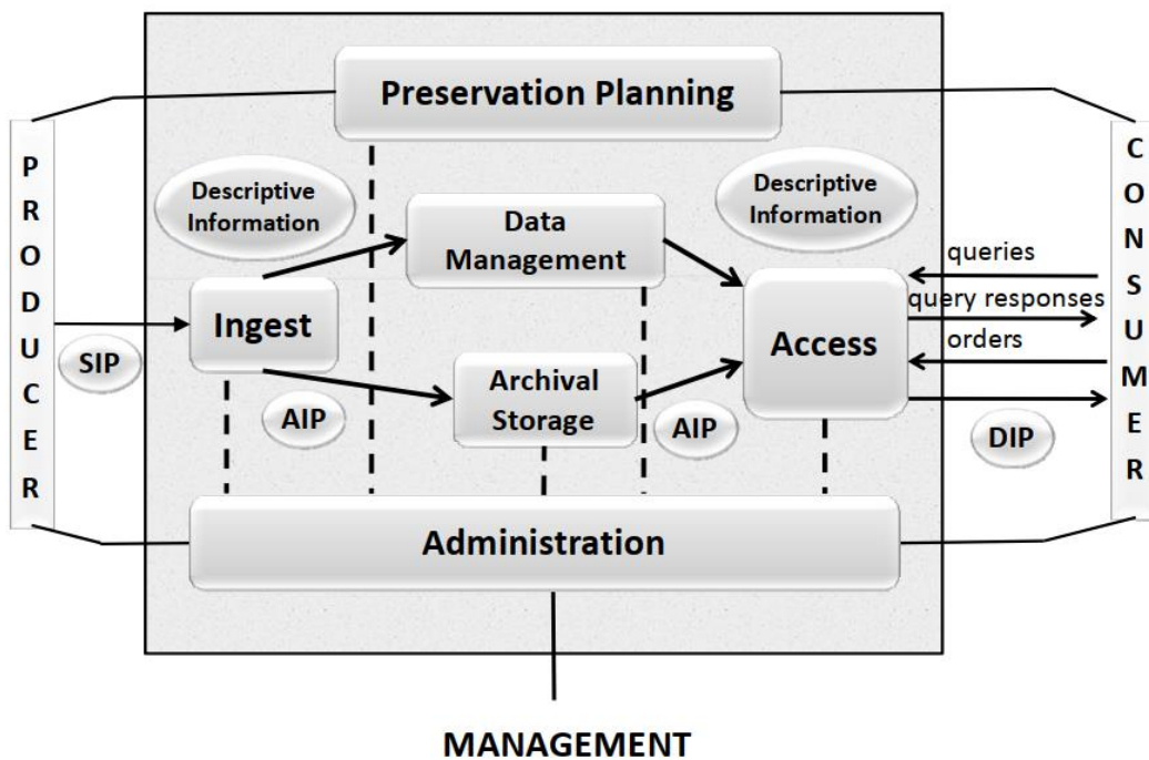
Abbildung 2: OAIS Functional Entities 2
