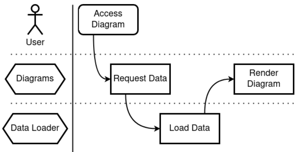
Figure 3.2: This flowchart describes the behavior when loading a diagram directly. As the diagram is unable to register with a data service, it will request the data directly from the data loader.
