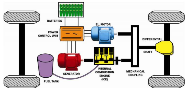
Figure 5: Series-Parallel Hybrid Electric Vehicle
