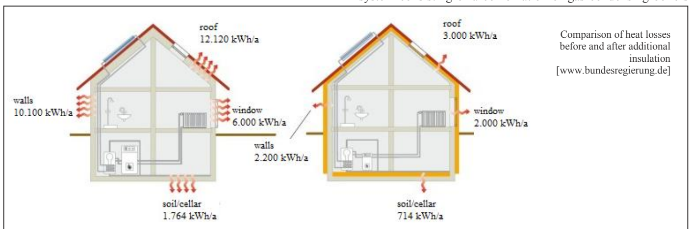
Figure 1: Comparison of heat losses
