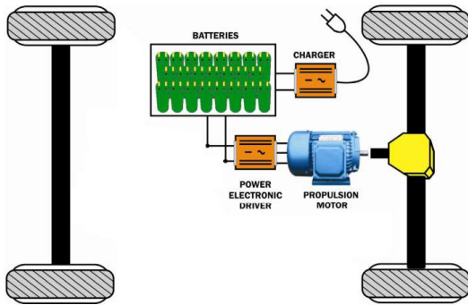
Figure 2: Battery Electric Vehicle
