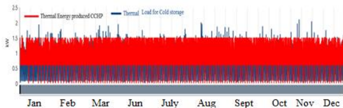
Fig. 17: Thermal Load and thermal generation by CCHP
