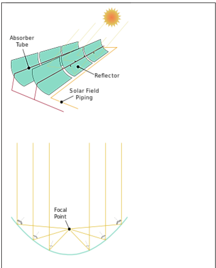
Fig. 4: Principle Illustration of the solar thermal process [1]
