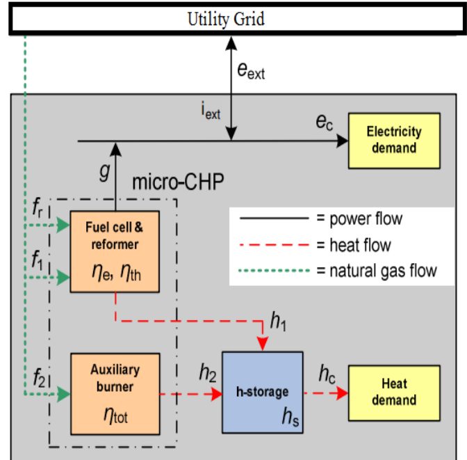
Fig. 4: Domestic \mu -CCHP System Control Scheme [20]
