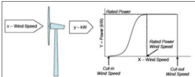
Figure 6: Power Curve [8]
