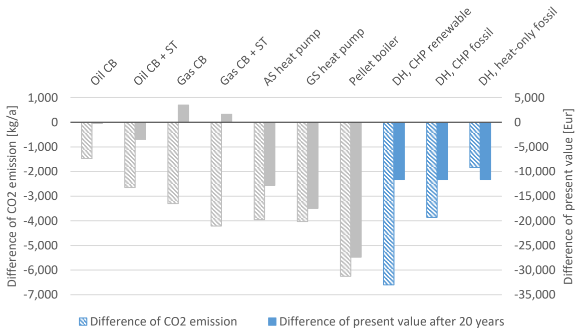
Figure 18 – Differences of CO 2 emissions and present value of a building’s heating system after 20 years in the event of replacing an outdated oil or gas boiler by a new heating system in a partly refurbished single-family house (Pfnür et al. 2016)
