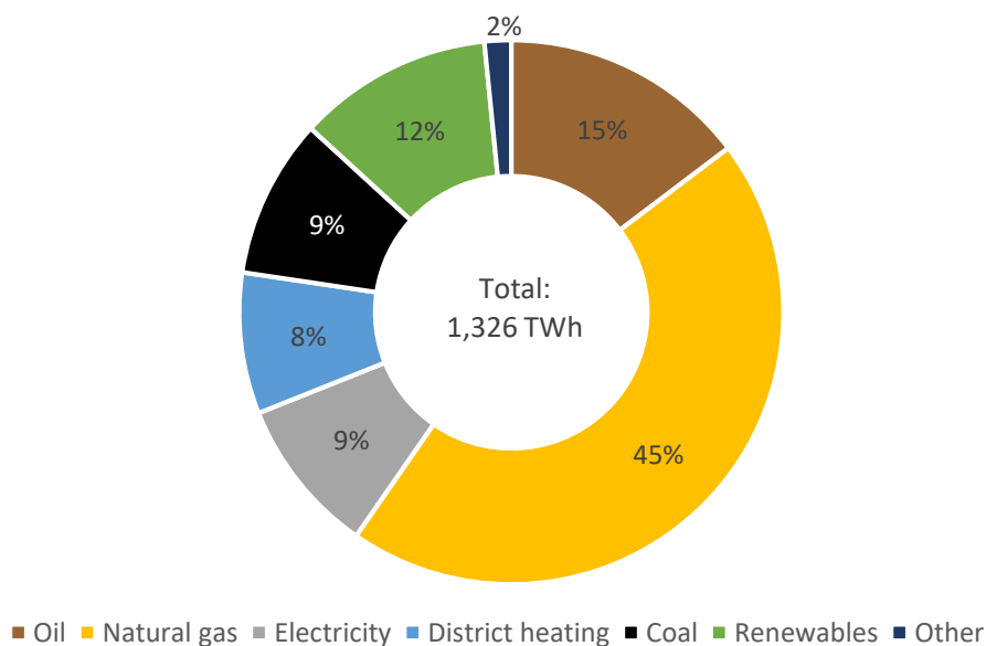
Figure 3 – Shares of fuel sources of total final energy consumption for heating over the sectors of households, TCS and industry in Germany 2018 (BMWi 2019a)
