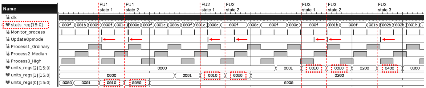
Fig. 5. Faults simulation performed over the platform, the units status register ( units_reg ) is incremented time to time simulating fault detection in the FUs. Numbers in the wave chart are in hexadecimal notation.
