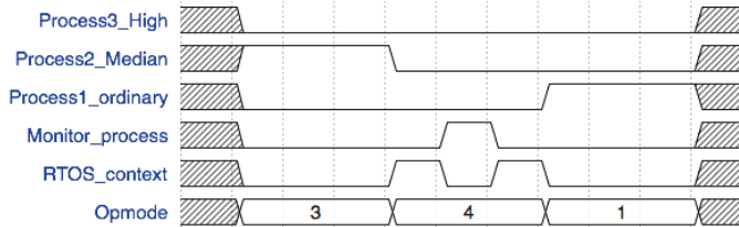
Fig. 4. Process switching time: switching between two application process and the Monitor process.
