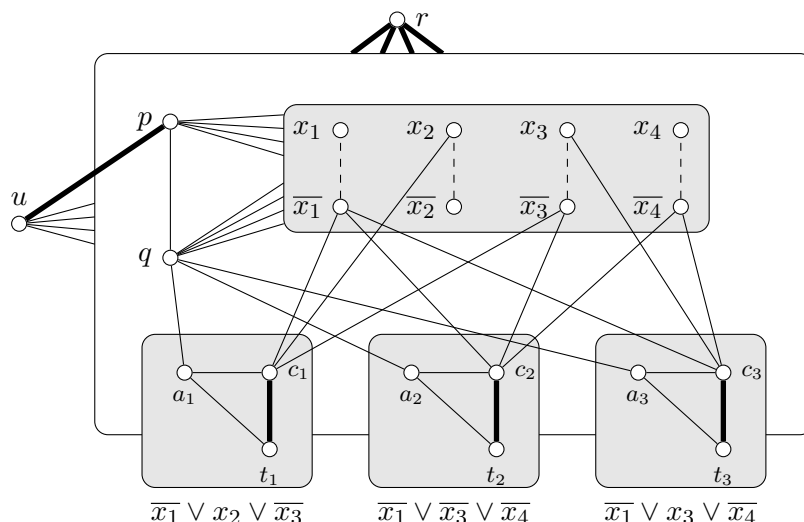
Figure 5.2: The \mathcal{NP} -completeness construction for the tree-recognition problem of LBFS. The depicted graph is G(\mathcal{I}) for \mathcal{I} = (\bar{x}_1 \vee x_2 \vee \bar{x}_3) \wedge (\bar{x}_1 \vee \bar{x}_3 \vee \bar{x}_4) \wedge (\bar{x}_1 \vee x_3 \vee \bar{x}_4) . In the box containing the literal vertices, only non-edges are displayed by dashed lines. The connection of a vertex with a box implies, that the vertex is connected to all vertices in this box. Tree edges are depicted by thick edges.
