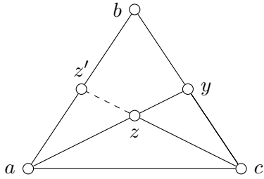
Figure 0.2: Peano Property and Pasch Property
