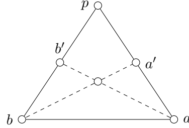
Figure 0.3: Peano Property and Pasch Property
