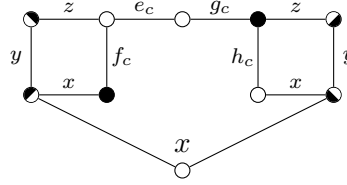
Figure 2.4: Gadget for the clause c = x \vee y \vee z
