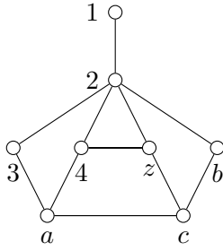
Figure 2.10: Example of a graph with a bad claw. On the right, one can see that the second \sigma_2 is not an AT-free order and \sigma_3 is not a bilateral AT-free order. In fact, this is an example of an AT-free graph that does not possess a bilateral AT-free ordering.
