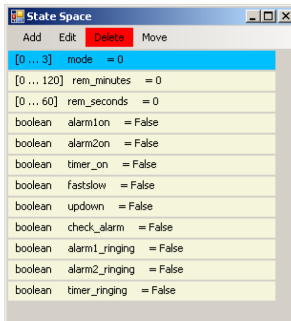
Figure 5.3: An example of the state space form
