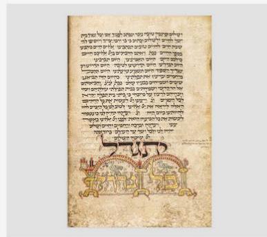
Amsterdam Mahzor
