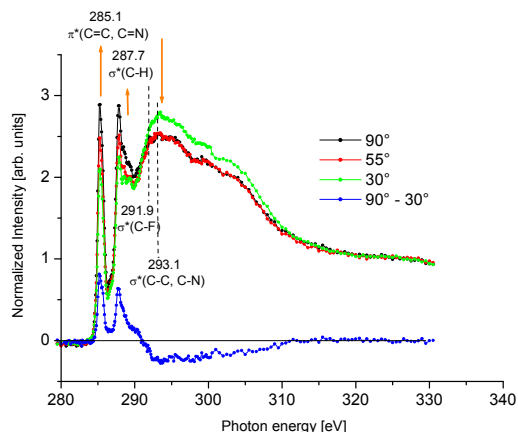
Figure 4.34. C K-edge NEXAFS at three different angles of incidence of linear polarized synchrotron light (30°, 55° and 90°) and the difference spectrum (90°-30°) for PFB derivatized 11-amino-1-undecanethiol ( 2 ) on Au.
