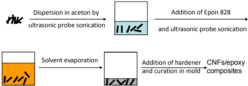
Figure 3.1 Scheme for the preparation of CNFs/epoxy nanocomposites.
