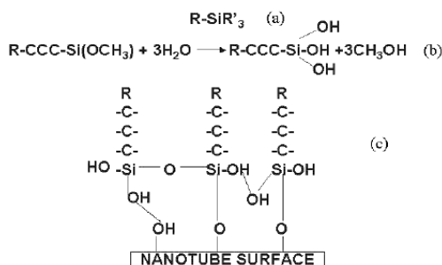
Figure 1.9 Scheme of the silanization process on CNTs [91].
