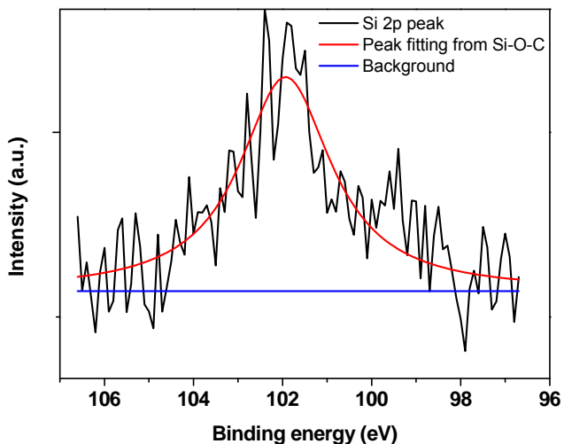
Figure 2.14 XPS Si 2p peak fitting of CNF-GS.
