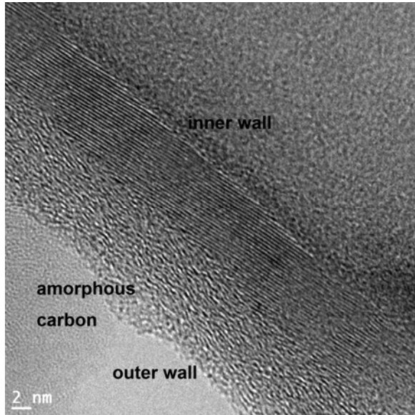
Figure 2.1 TEM picture of original CNFs.
