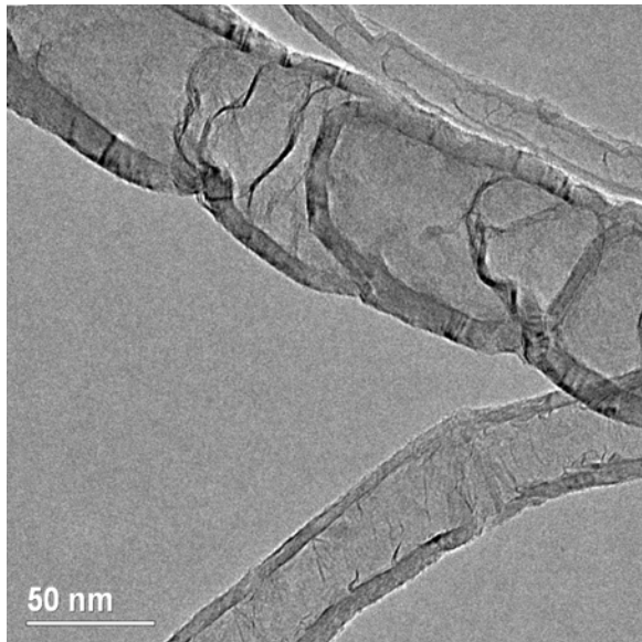
Figure 2.2 TEM picture of pristine MWCNTs.
