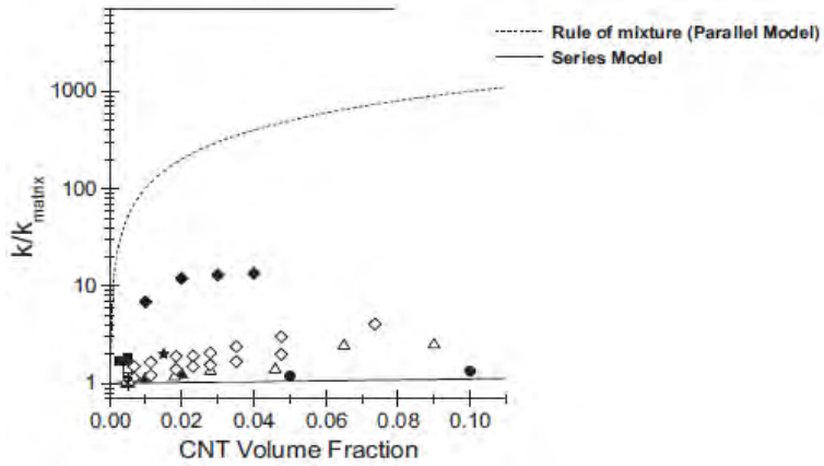
Figure 1.8 The enhancement of thermal conductivity of composites compared to that of pure polymer as a function of CNT volume fraction [80].
