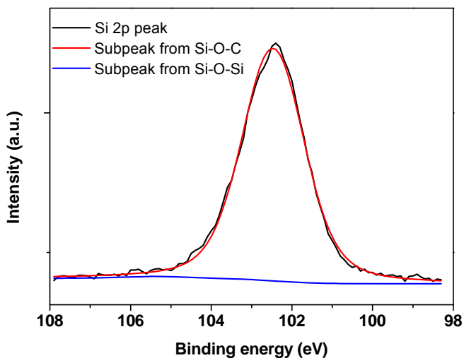
Figure 2.27 XPS Si 2p peak fitting of CNF-I-AP.
