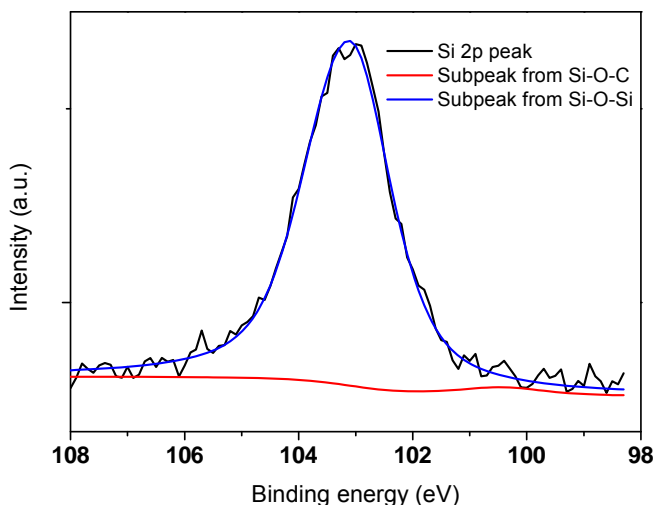
Figure 2.36 XPS Si 2p peak fitting of MWCNT-PMH-N-AP.
