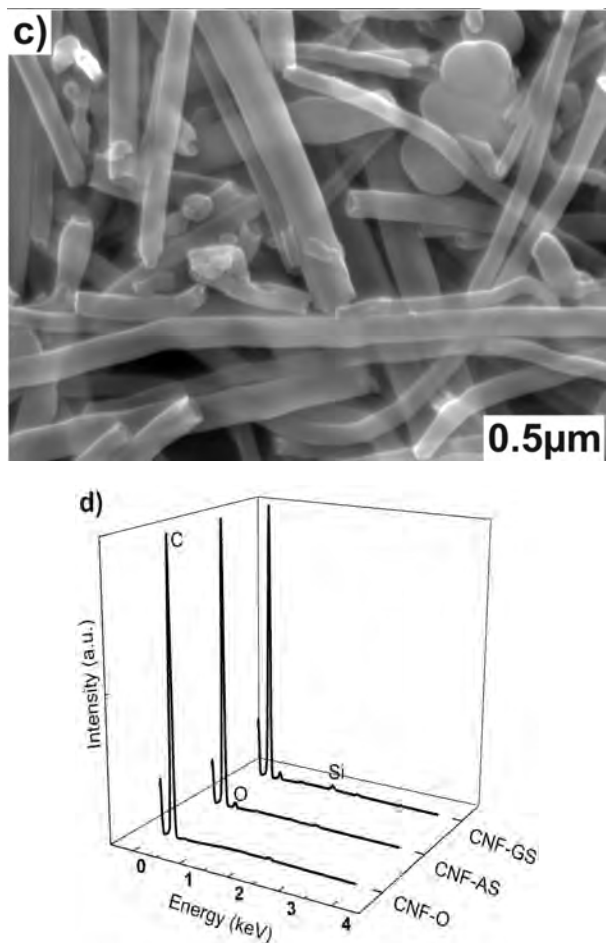
Figure 2.16 SEM of a) original CNFs (CNF-O), b) oxidized CNF (CNF-AS), c) silanized CNFs (CNF-GS); and d) EDX analysis of CNFs.
