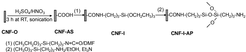
Figure 2.6 Sketch for the silanization process of CNFs with IPTES and APTMS.
