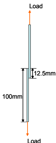
Figure 3.4 Scheme for the measurement of the tensile shear strength based on EN 1465.
