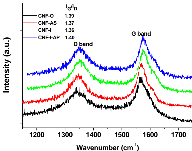
Figure 2.31 Raman spectra of silanized CNFs (CNF-I, CNF-I-AP) compared with original CNFs (CNF-O) and oxidized CNFs (CNF-AS).
