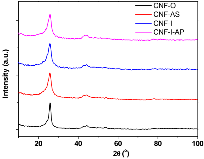
Figure 2.30 XRD patterns of CNFs before and after chemical treatments in the two-silanzation procedure.
