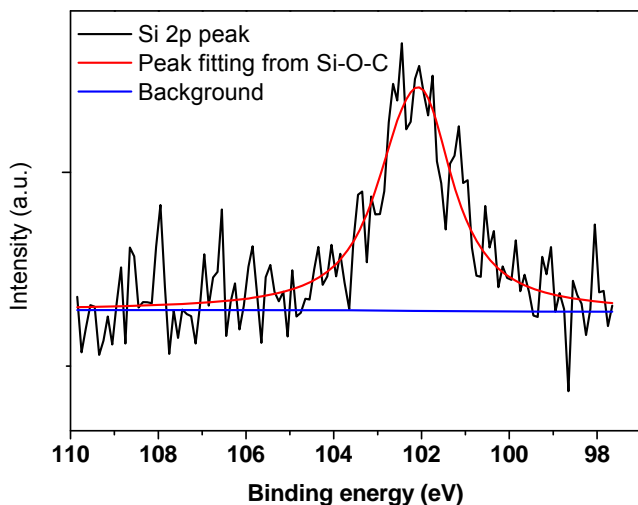
Figure 2.26 XPS Si 2p peak fitting of CNF-I.
