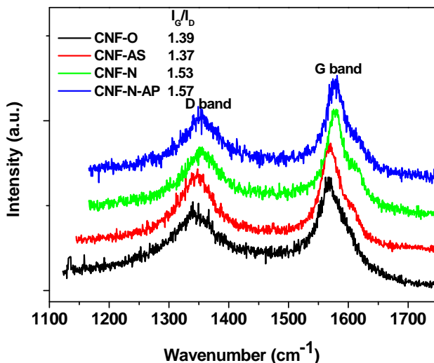
Figure 2.24 Raman spectra of CNF-N-AP compared with the original CNFs (CNF-O), oxidized CNFs (CNF-AS) and reduced CNFs (CNF-N).
