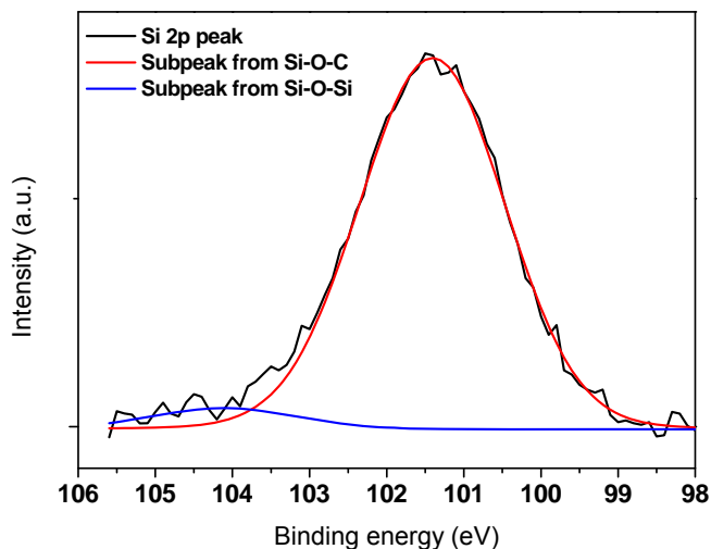
Figure 2.21 XPS Si 2p peak fitting of CNF-N-AP.
