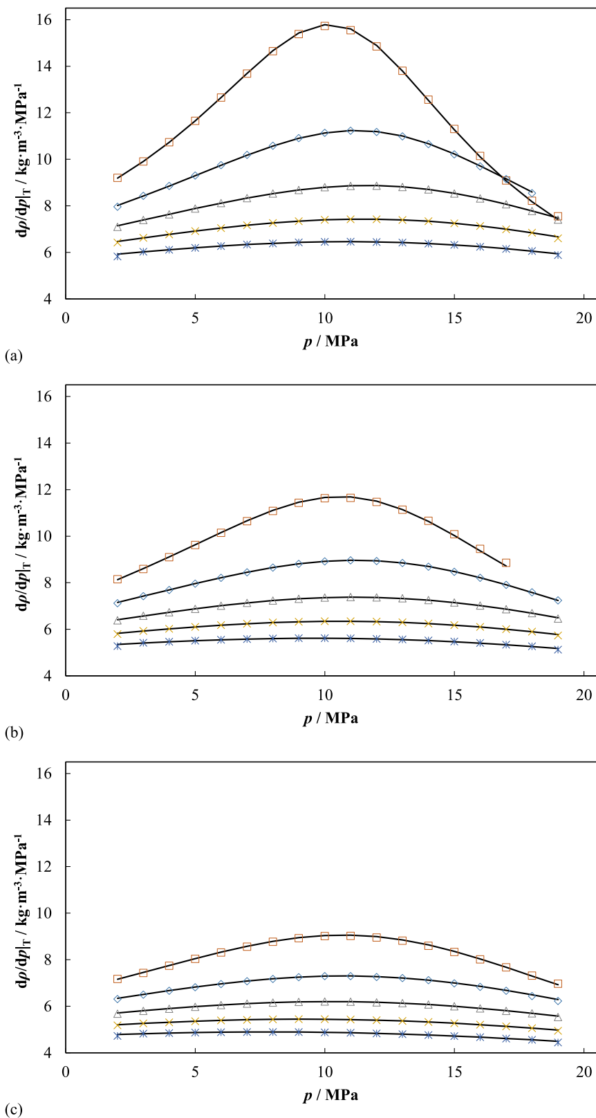
Fig. 5. Derived \left. \frac{\partial \rho_{\text{exp}}}{\partial p} \right|_T values of (a) G 431, (b) G 453 (G 431 + 10 % H 2 ), and (c) G 454 (G 431 + 20 % H 2 ) mixtures as a function of the pressure for different temperatures: \square 250 K, \diamond 275 K, \triangle 300 K, \times 325 K, \circ 350 K. Solid lines indicate the \left. \frac{\partial \rho_{\text{EoS}}}{\partial p} \right|_T values calculated from the improved-GERG-2008 EoS [44–46].
