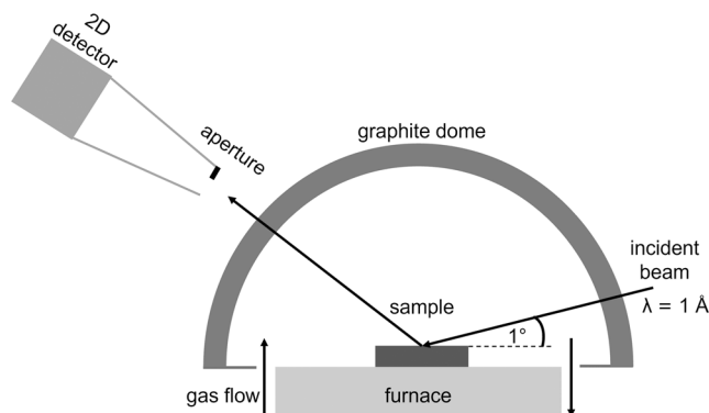
FIGURE 2 Sketch of experimental setup. The incident beam passes through a graphite dome to graze the sample at a 1° angle. During the experiment, the sample is heated via a furnace, and gas flows through the dome. The diffracted beam is then recorded by a 2D detector.
